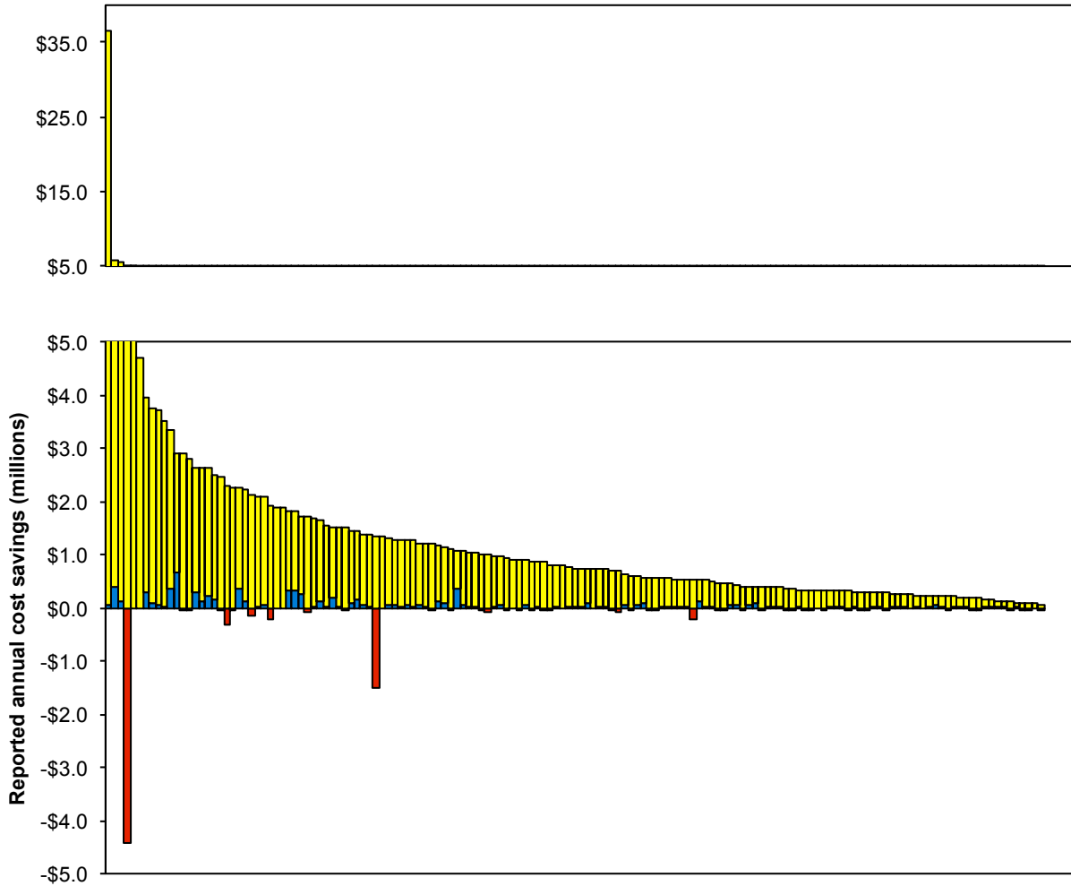
Fig. 5. Reported and estimated annual cost savings from 151 DOE ESPC projects. Reported cost savings above the estimated amount are shown in blue, and reported savings below the estimated amount are shown in red. Where reported cost savings equals or exceeds the estimated savings, the height of the yellow bar is equal to the estimated savings. Where reported cost savings is less than the estimated amount, the estimated savings is equal to the height of the yellow and red bars combined.
