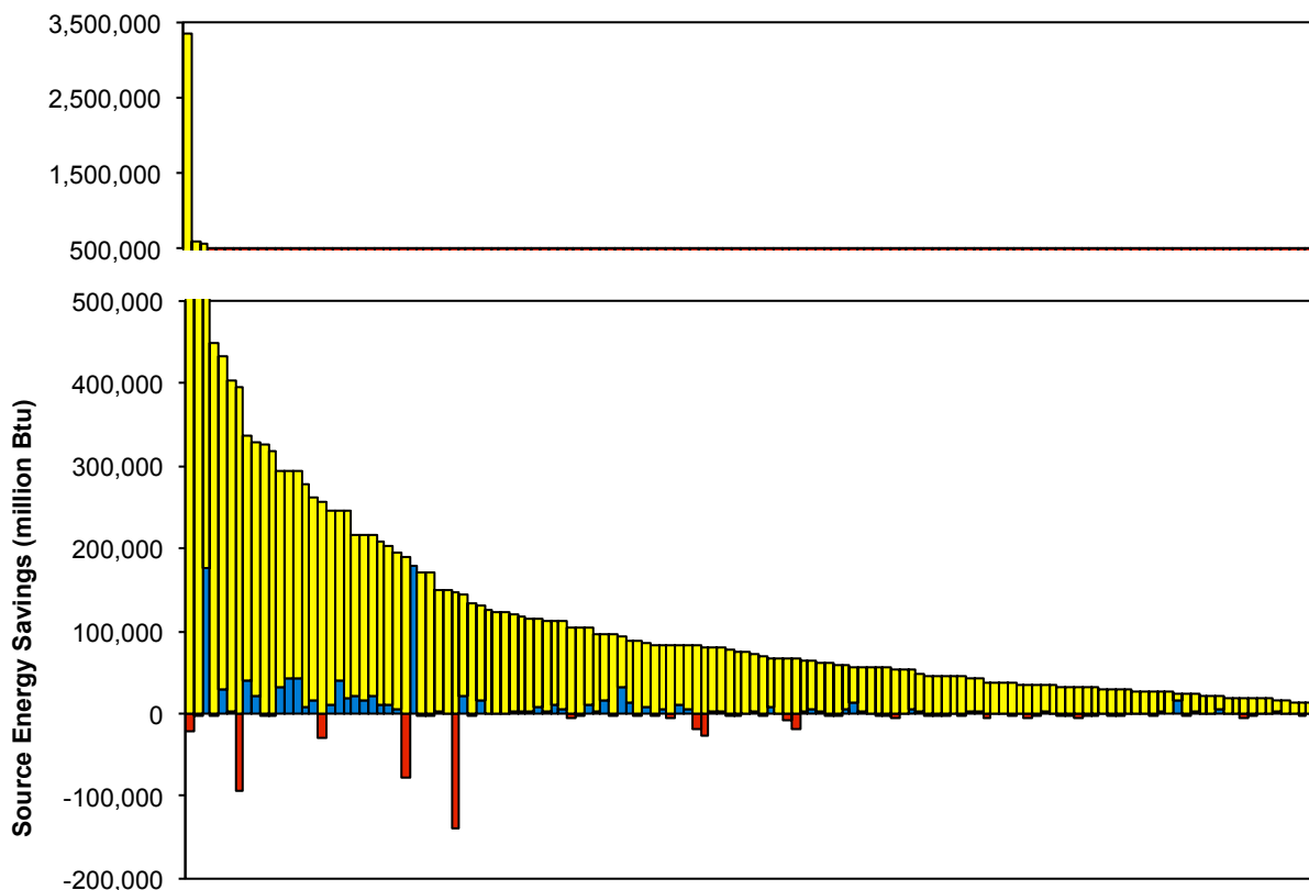
Fig. 7. Annual source energy savings from 151 ongoing DOE ESPC projects. Reported energy savings greater than the estimated savings are shown in blue, and reported energy savings less than the estimated savings are shown in red. Where no shortfall occurs, the yellow bar is the amount of the estimated savings. Where a shortfall occurs, the amount of the estimated savings is the sum of the heights of the yellow and red bars.
