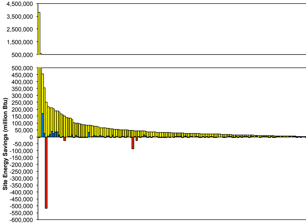
Fig. 6. Annual site energy savings from 151 ongoing DOE ESPC projects. Reported energy savings greater than the estimated savings are shown in blue, and reported energy savings less than the estimated savings are shown in red. Where no shortfall occurs, the yellow bar is the amount of the estimated energy savings. Where a shortfall occurs, the amount of the estimated energy savings is the sum of the heights of the yellow and red bars.
