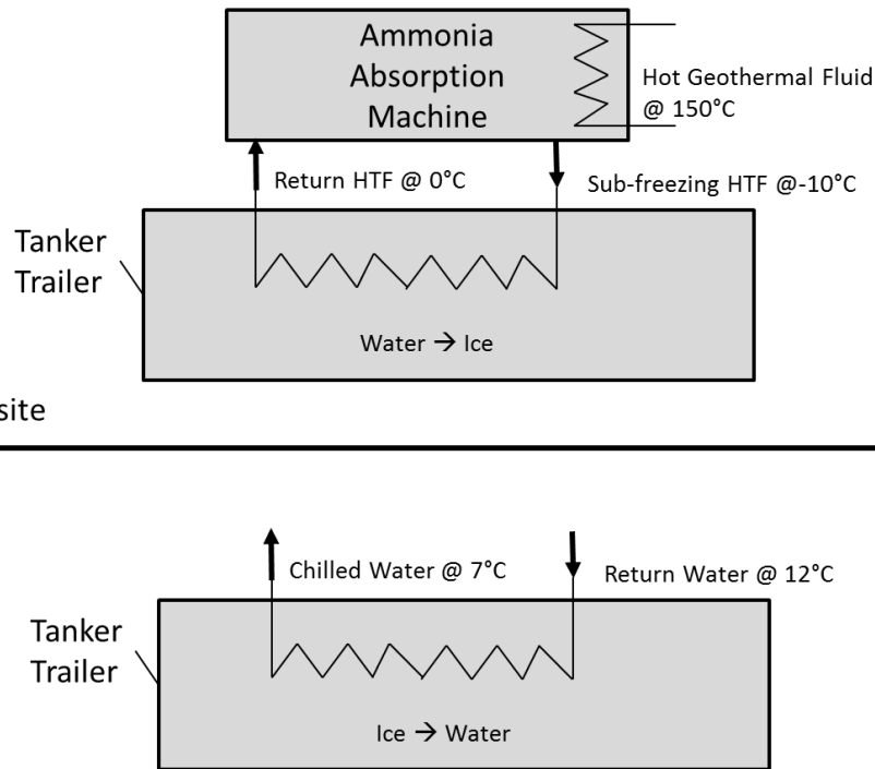
Fig. 14. Ice storage system operation cycle.
