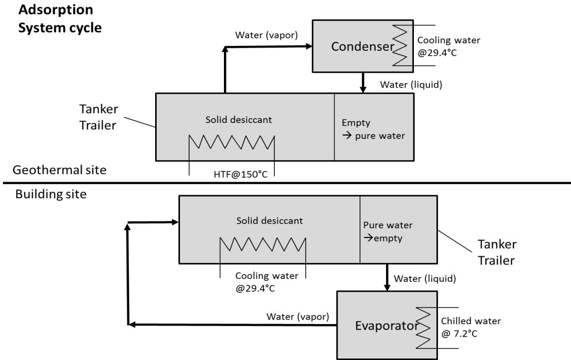
Fig. 11. Adsorption system operation cycle.
