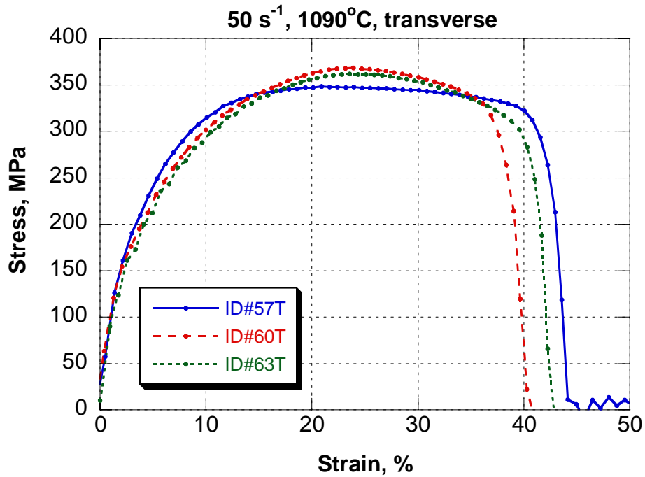
Fig. 23. Stress-strain curves at 50 \text{ s}^{-1} and 1090^\circ\text{C} , transverse specimen orientation.
