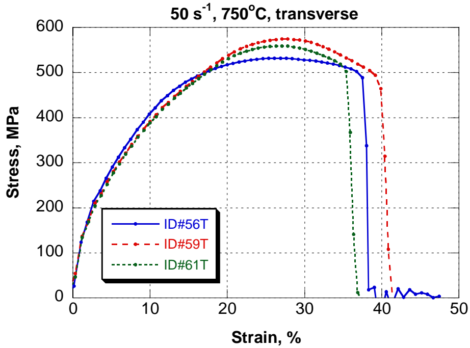
Fig. 22. Stress-strain curves at 50 \text{ s}^{-1} and 750^\circ\text{C} , transverse specimen orientation.
