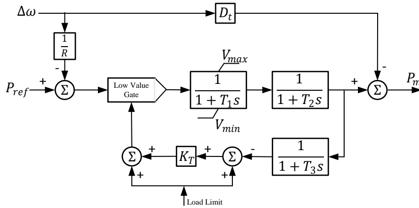
Fig. 7. Control diagram of GAST.
