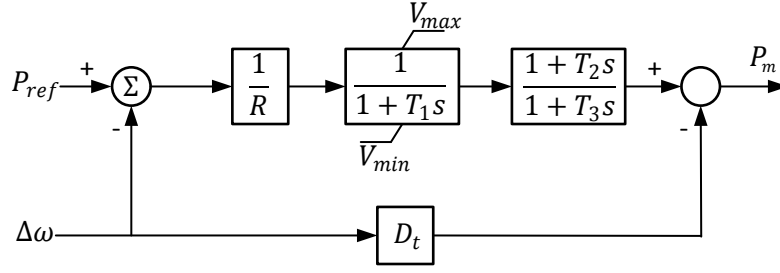
Fig. 6. Control diagram of TGOV1.
