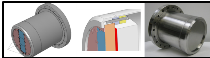
Figure 5. Design of the large field-of-view detector and photograph of the prototype detector with a stainless steel blank substituted for the fiber-optic window.
