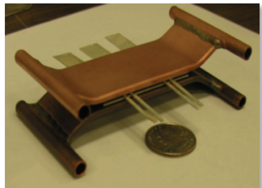
Planar_Bond_All photo showing double-sided planar interconnections and integrated mini-coolers.
