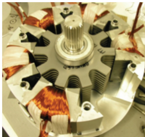
Partially assembled prototype showing yoke-wound stator coils.
