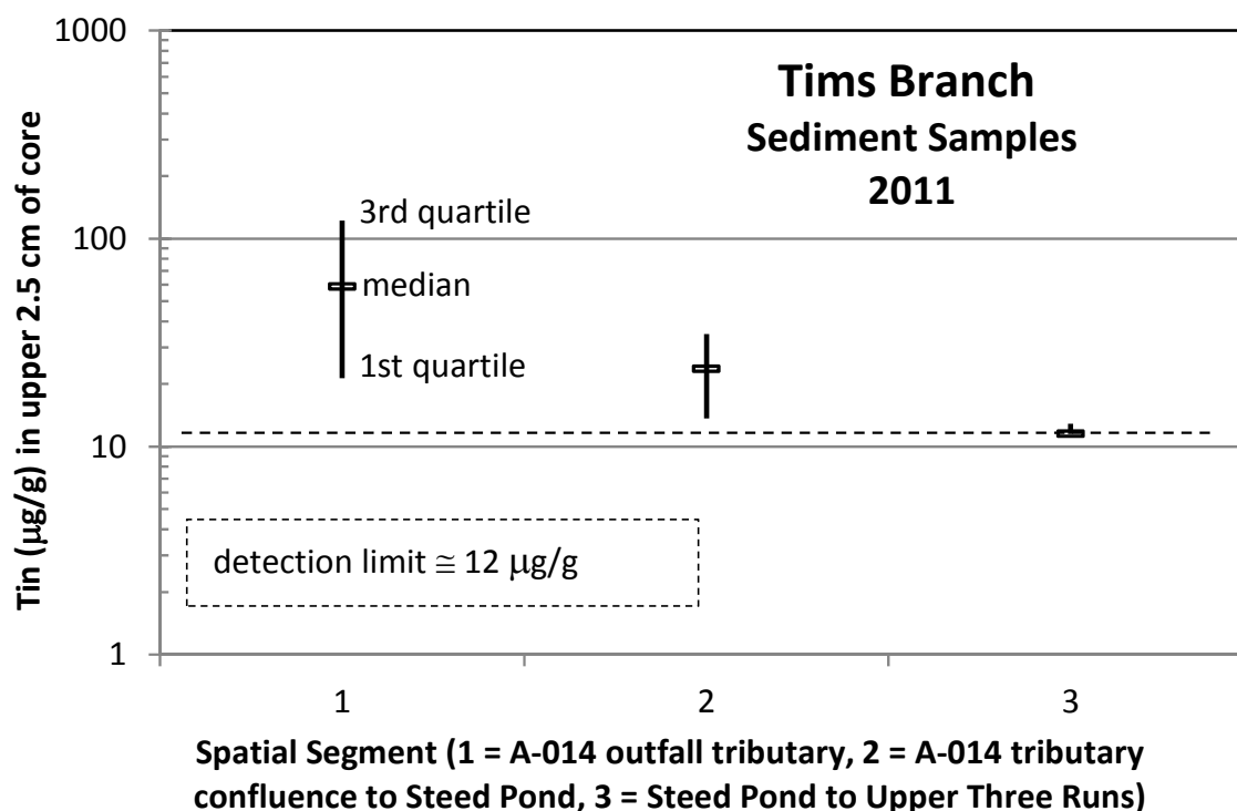
Figure 12. Sediment concentrations for tin in M Area outfall tributary and Tims Branch
