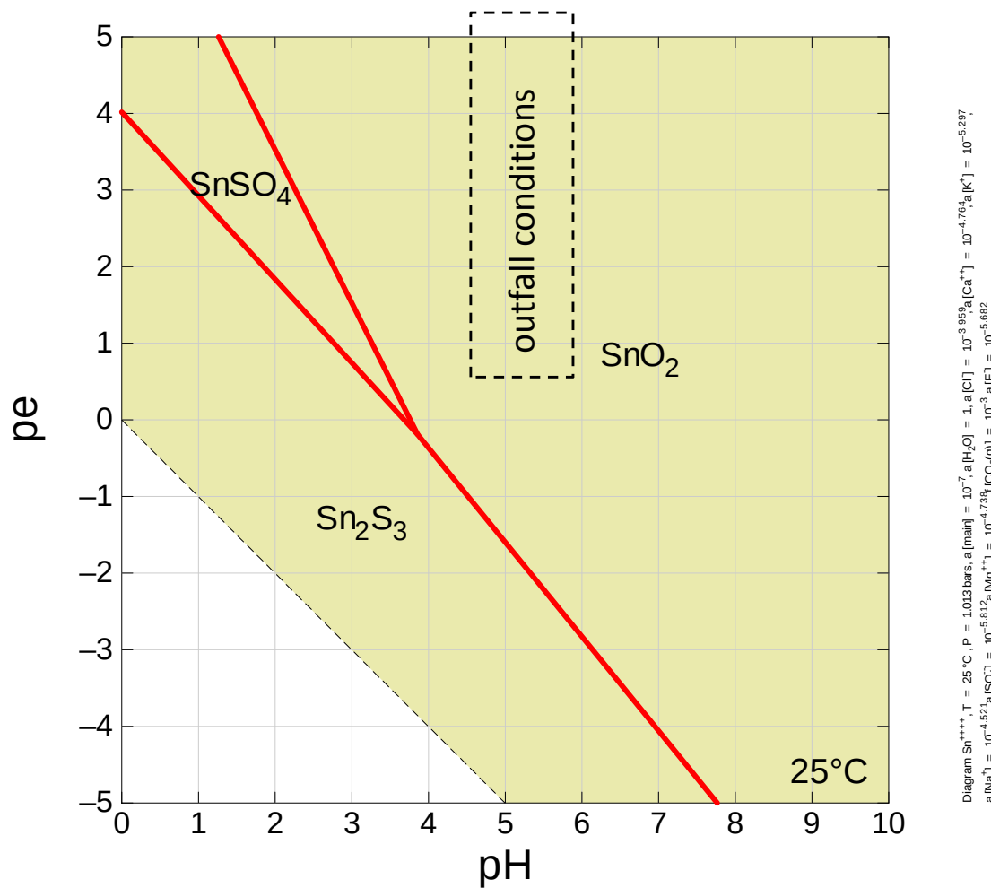
Figure 8. Geochemical speciation of tin for outfall conditions
