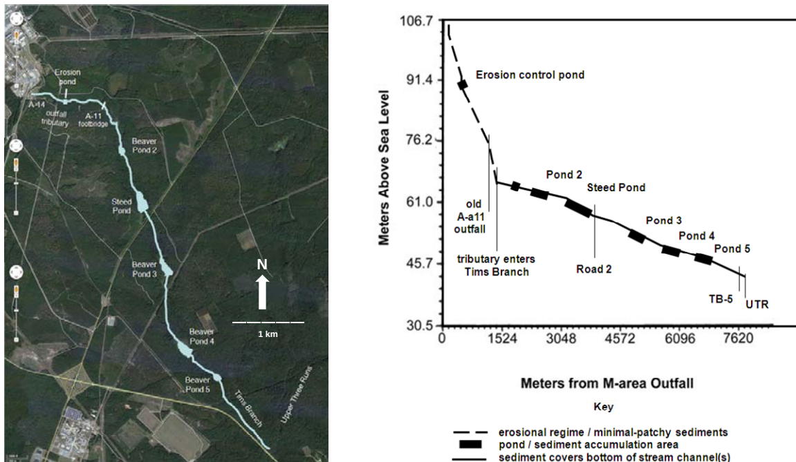
Figure 7. Morphology of M Area outfall tributary and Tims Branch
