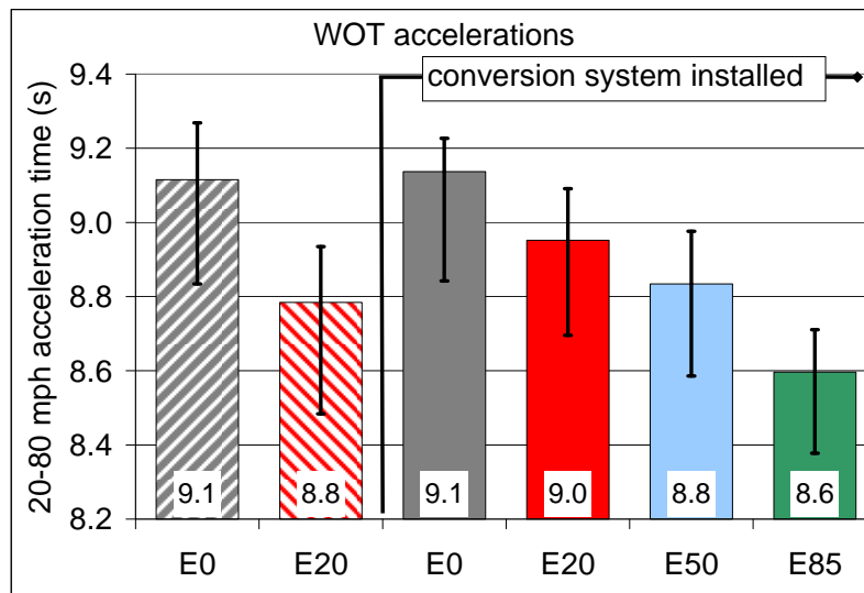
Fig. 11. WOT acceleration times from 20 mph to 80 mph for all fuels. Range bars show maximum and minimum test results.
