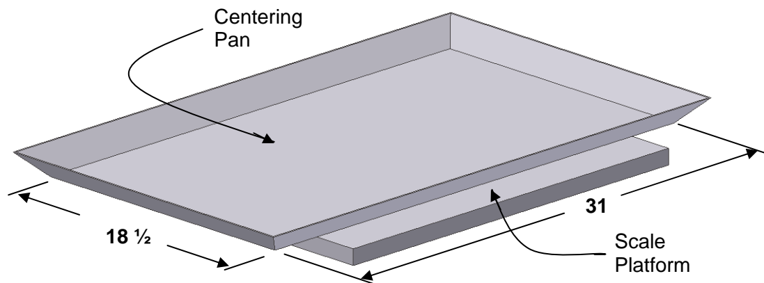
Fig. 6. Centering pan for 250-kg capacity scales.
