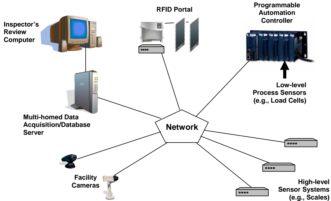
Fig. 5. Data collection system architecture.
