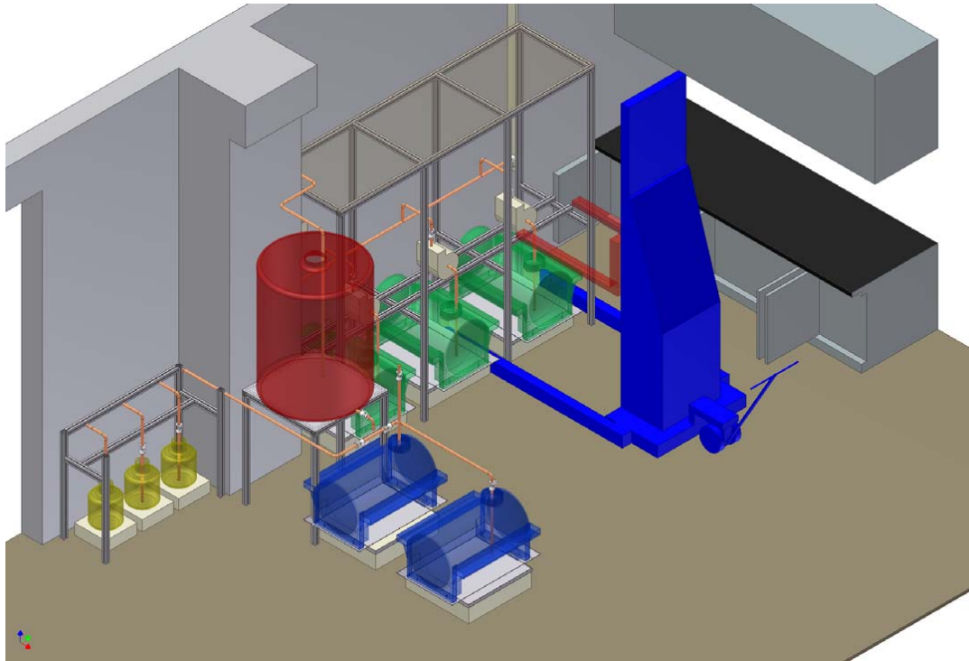
Fig. 2. Color-coded diagram of mock F&W system—with green feed tanks, yellow product tanks, blue tails (or waste) tanks, and a red process tank.
