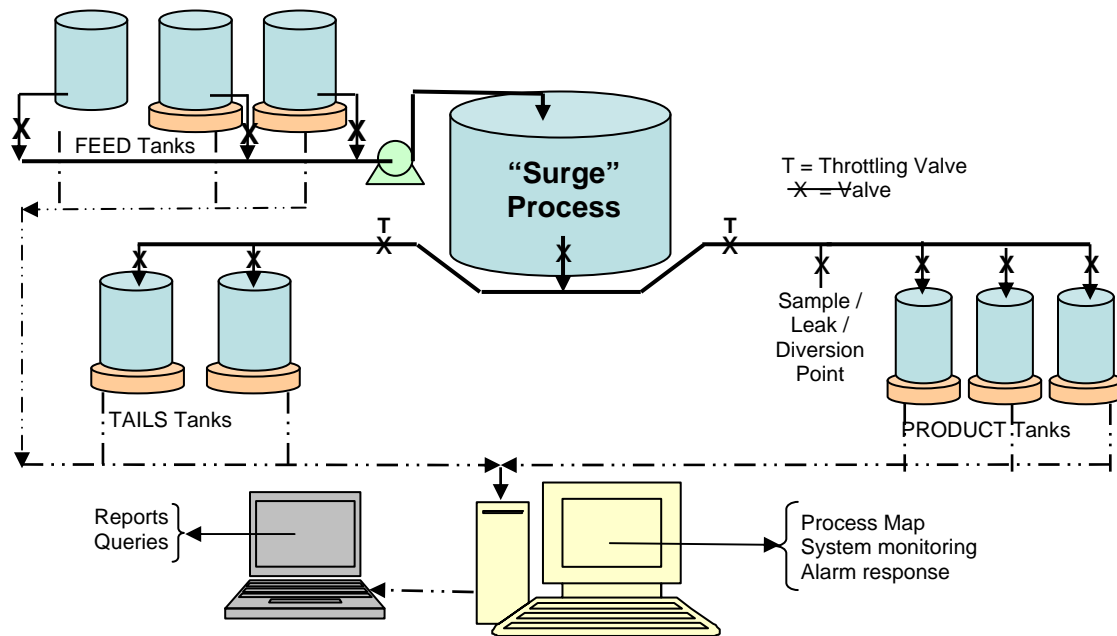
Fig. 7. Process schematic for mock F&W system. [Each tank is shown resting on a dedicated scale (depicted in tan).]
