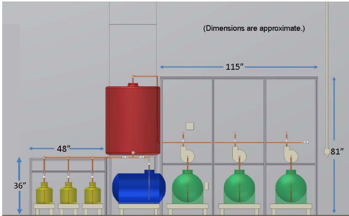
Fig. 4. Elevation view of mock F&W system diagram.
