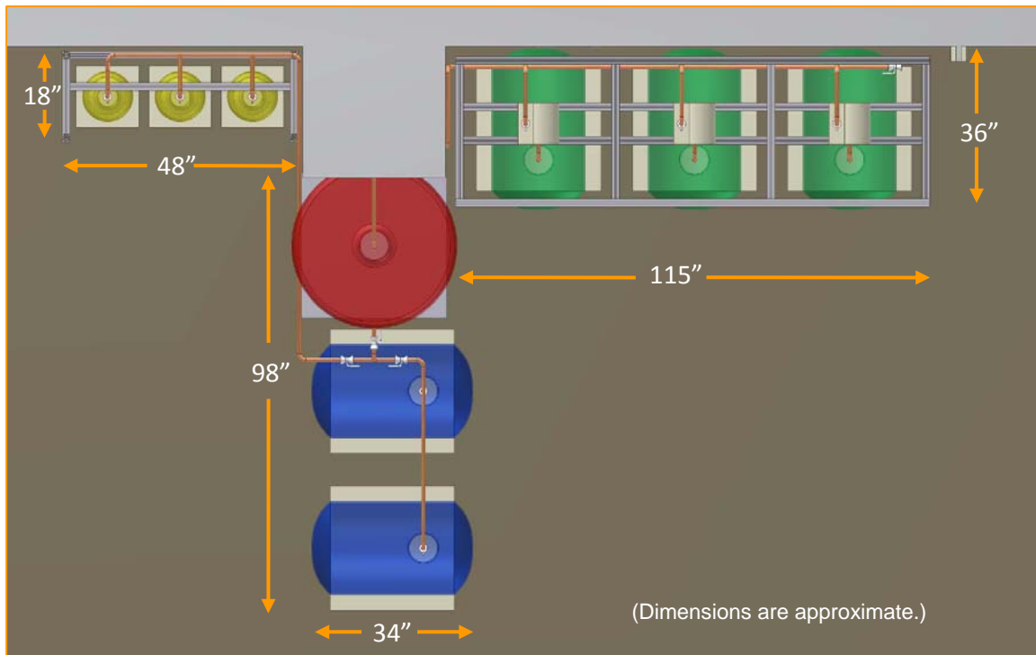
Fig. 3. Plan view of mock F&W system diagram.
