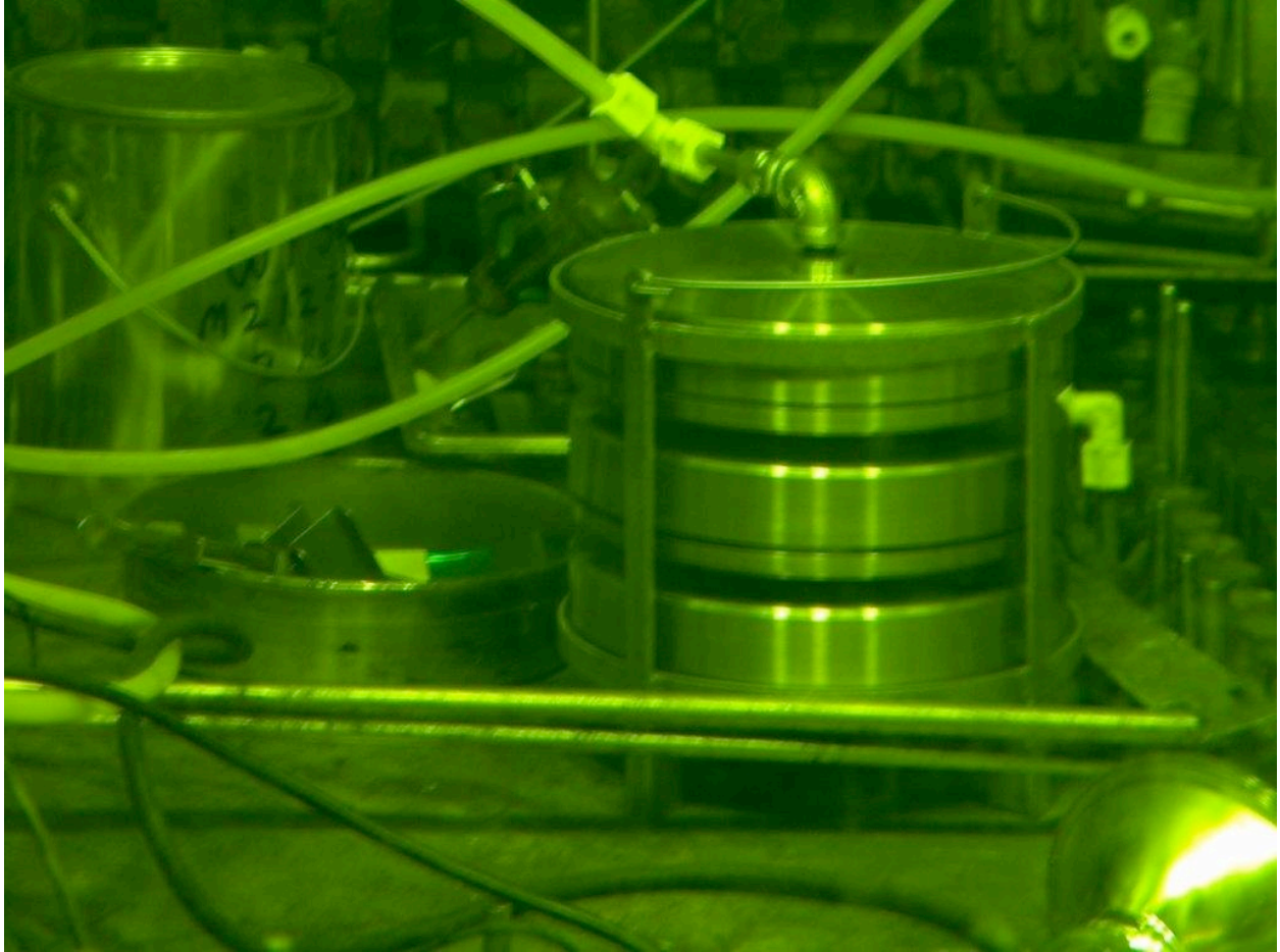
Figure 1. Photograph of the undissolved solids recovery equipment as installed in the hot cell (Cubicle 5, Bldg. 7920).
