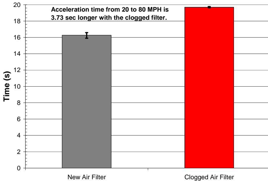
Fig. 3.15. Acceleration time for 1972 Pontiac Grandville during WOT tests. Data are averaged over the three CRC-E60 accelerations from 20 to 80 mph with the throttle at 100%. Range bars show the minimum and maximum for each data set.
