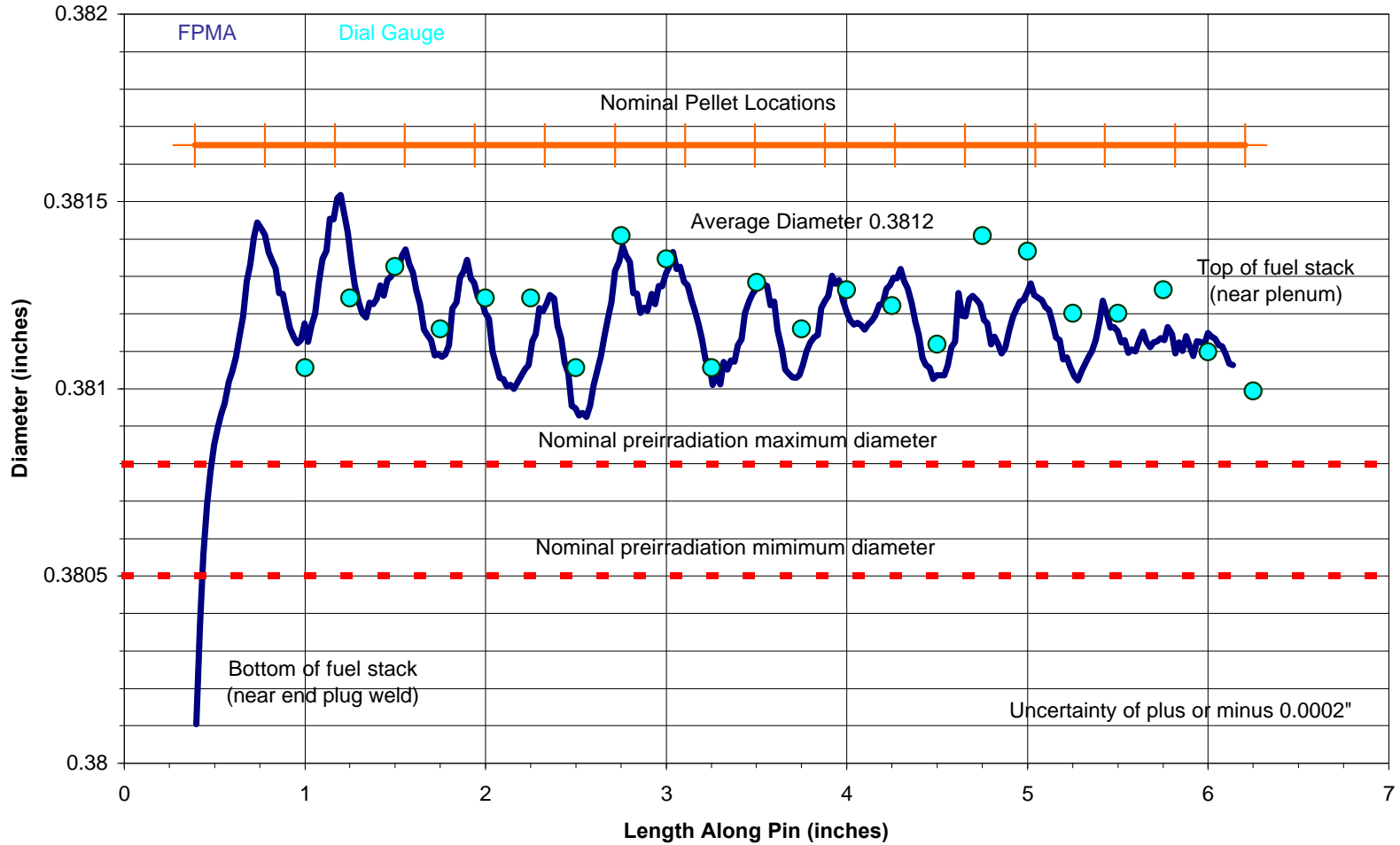
Figure 13. Results of both FPMA and dial indicator/V block measurements for Fuel Pin 13. Note the alignment between the graph peaks and the pellet locations
