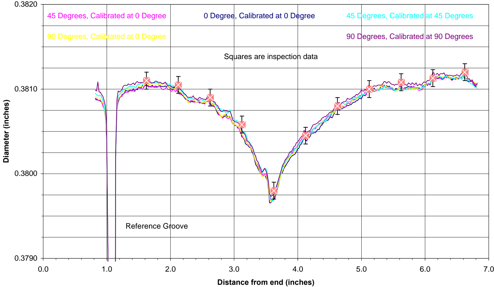
Figure 8. Diameter measurement results at different vise angles both with and without recalibration.
