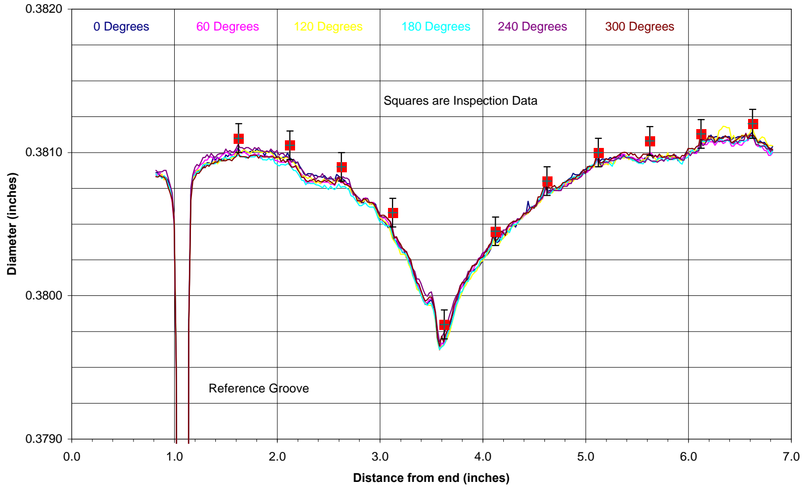
Figure 9. Diameter measurement results from 6 view angles and inspection data for the dummy fuel pin.
