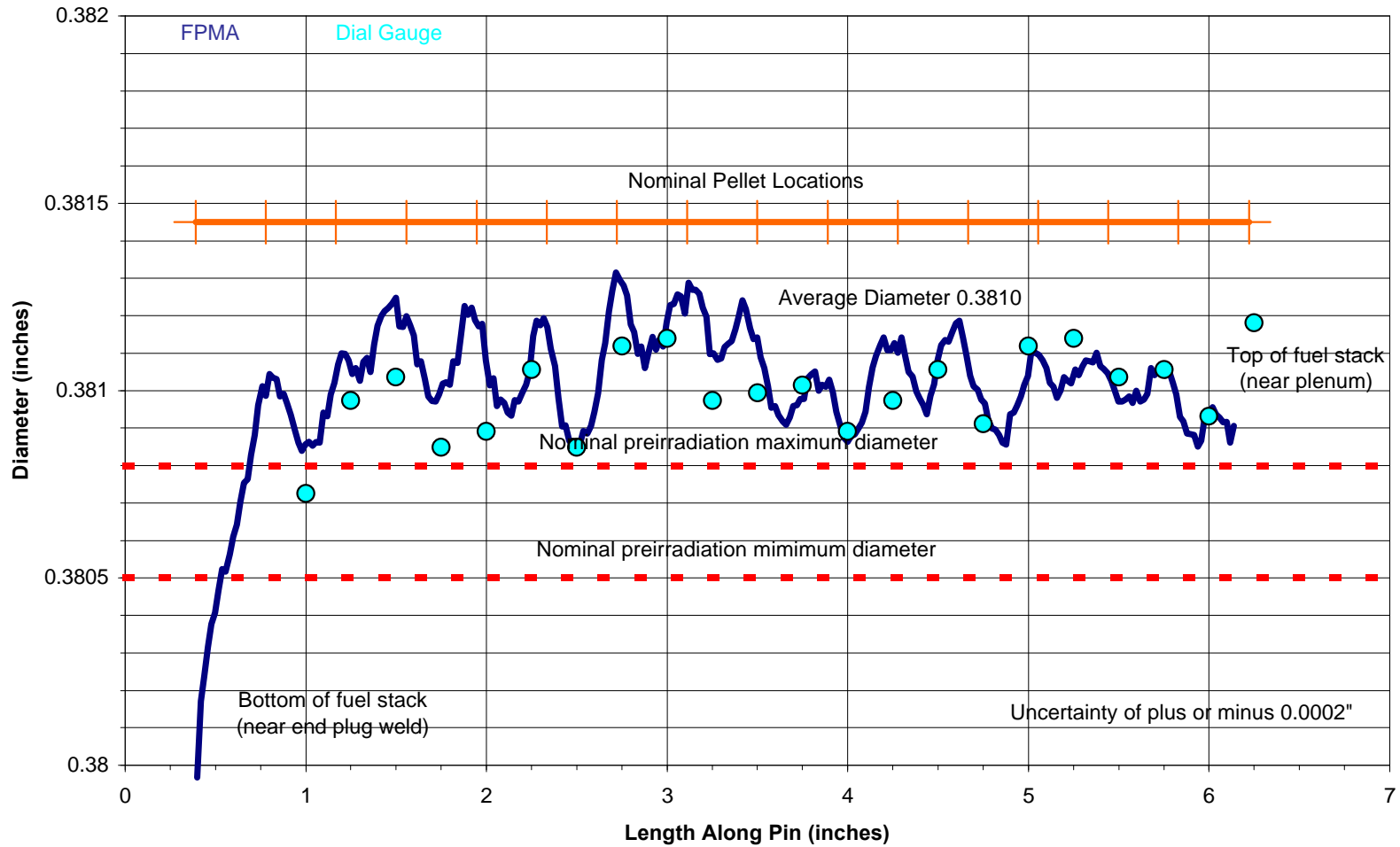
Figure 12. Results of both FPMA and dial indicator/V block measurements for Fuel Pin 6. Note the alignment between the graph peaks and the pellet locations.
