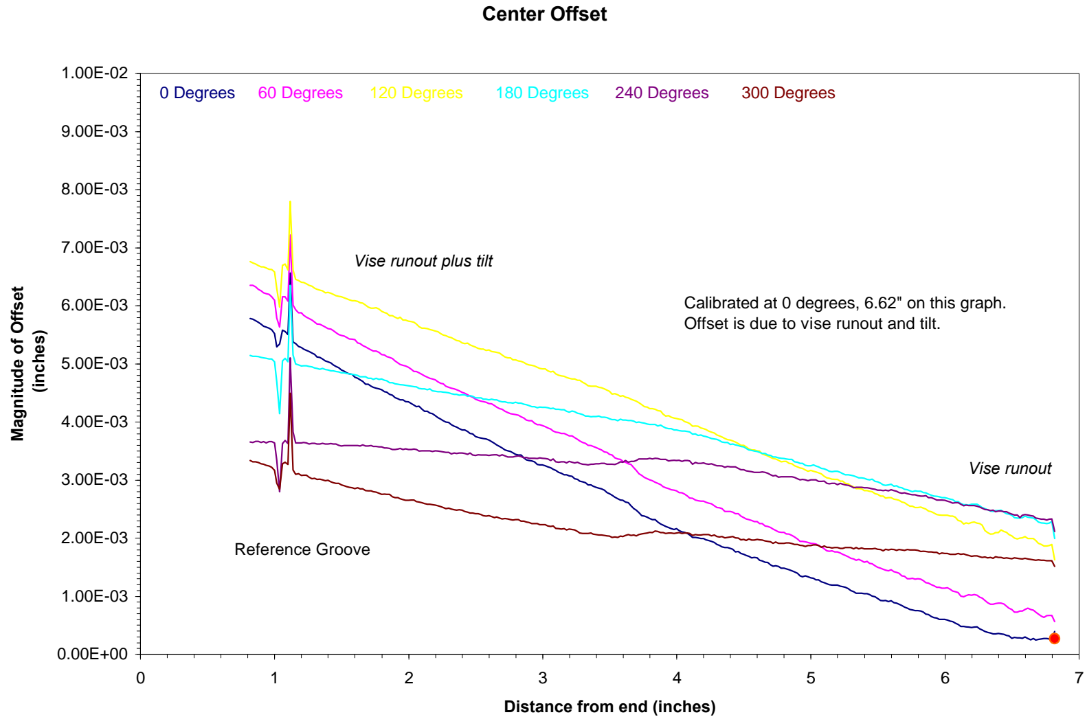
Figure 10. Computed offsets for the different vise angles. The red dot is the calibration position before inserting the dummy fuel pin (0 degrees).
