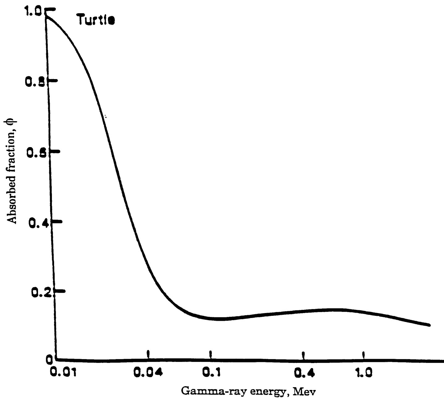
Fig. A.3 Derived absorbed fractions as a function of \gamma ray energy (turtle).
