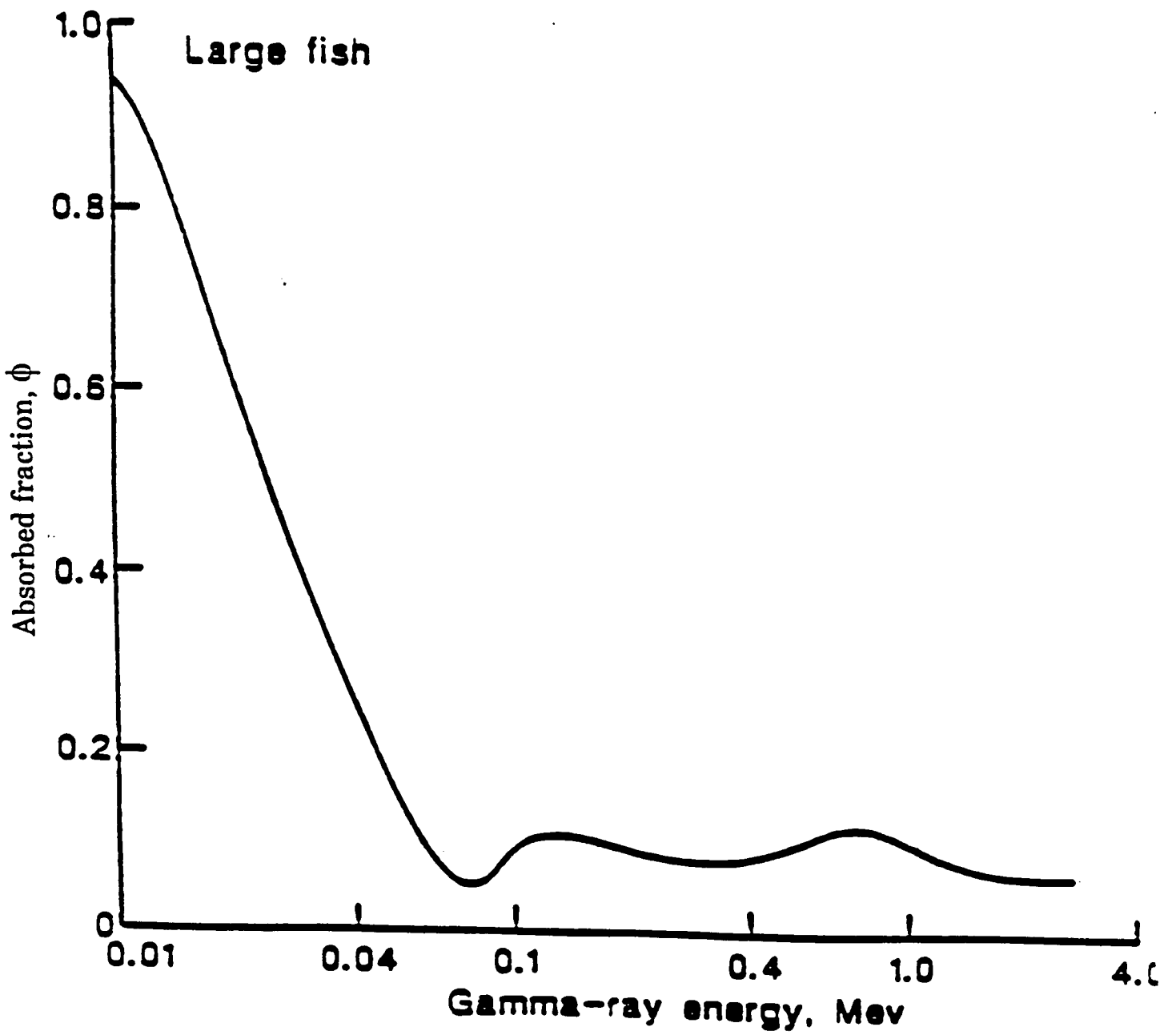
Fig. A.2 Derived absorbed fractions as a function of \gamma -ray energy (large fish).
