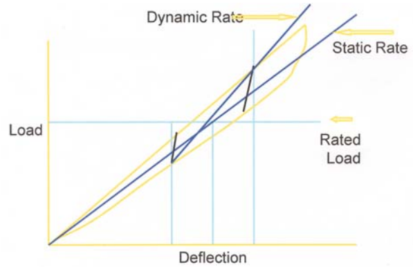
Fig. 5. Hysteresis in Multiple Leaf Springs (Courtesy of Hendrickson International)
