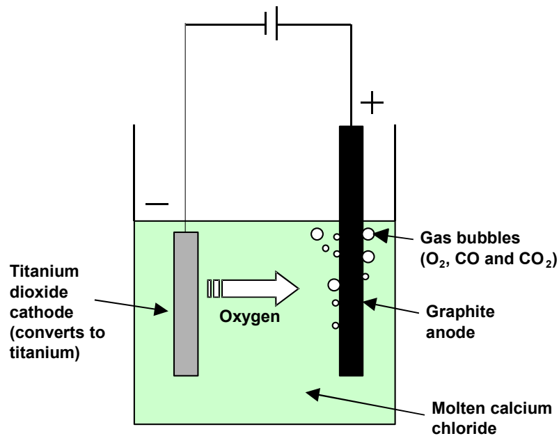
Fig. 14. Schematic Description of the FFC-Cambridge Process Reduction Step 18
