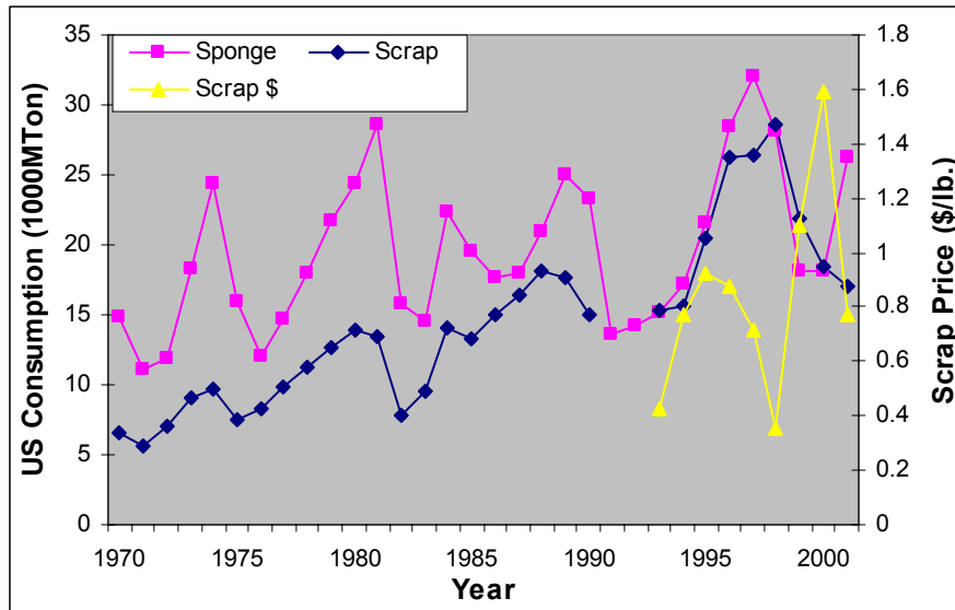
Fig. 12 Annual U.S. Ti Scrap and Sponge Consumption and Scrap Price 9
