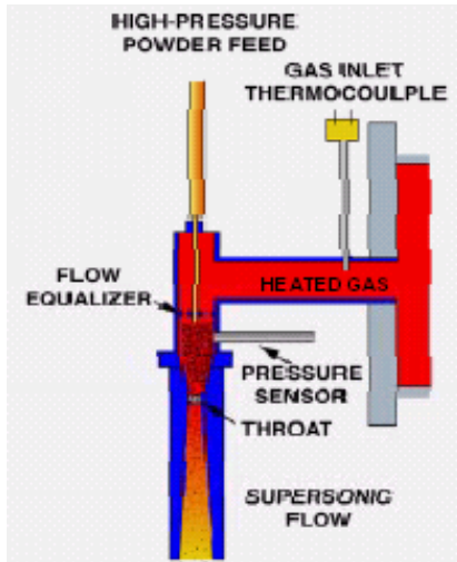
Fig. 20. Cold Spray Process (Courtesy Sandia Nat'l. Lab.)
