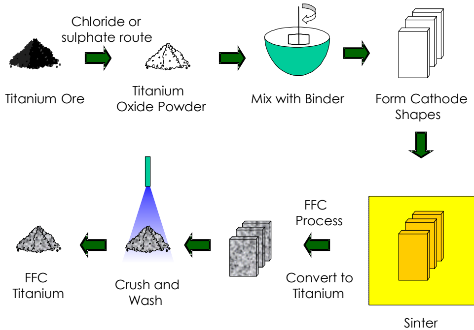
Fig. 13. Schematic Description of the FFC-Cambridge Process 18
