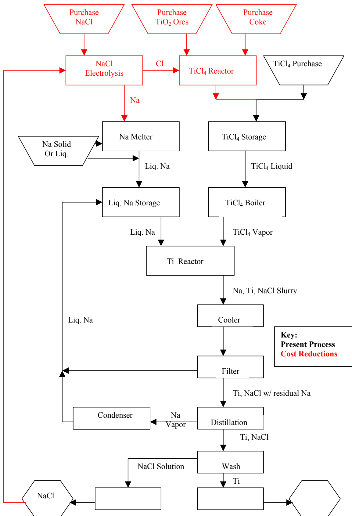
Fig. 15. Schematic Description of the ITP Process 26
