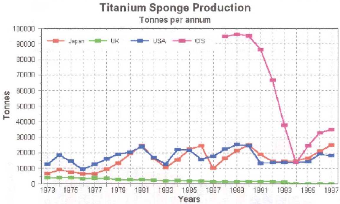
Figure 8. Variation in Titanium Sponge Production 18
