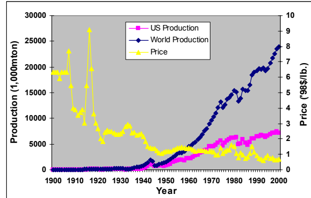
Fig. 11. Production and Price History for Aluminum 20
