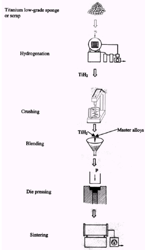
Courtesy of U. Idaho / ADMA Fig. 16. The Hydride – Dehydride Process
