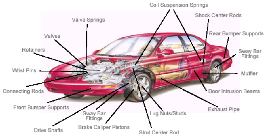
Fig. 22. Candidate Ti Applications Identified by TIMET Automotive Division (Courtesy TIMET Automotive)
