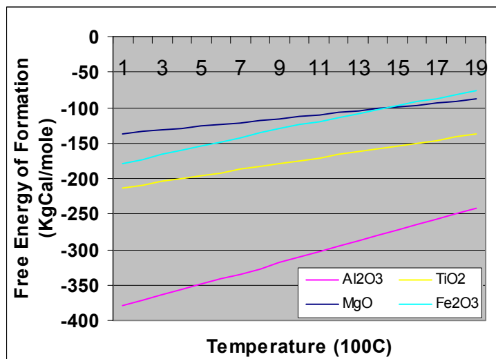
Fig. 7. Free Energy of Formation of Oxides 14
