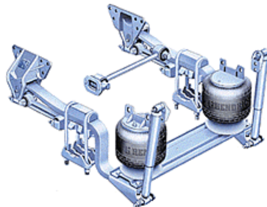
Fig. 3. Heavy-Duty Truck Suspension (Courtesy of Hendrickson International)
