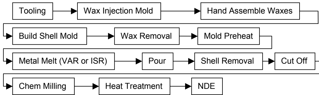
Fig. 6. Schematic Diagram of Turbocharger Rotor Investment Casting
