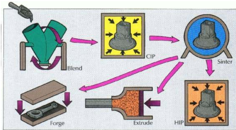
Fig. 18 The Dynamet CermeTi® Process (Courtesy of Dynamet Technology, Inc.)
