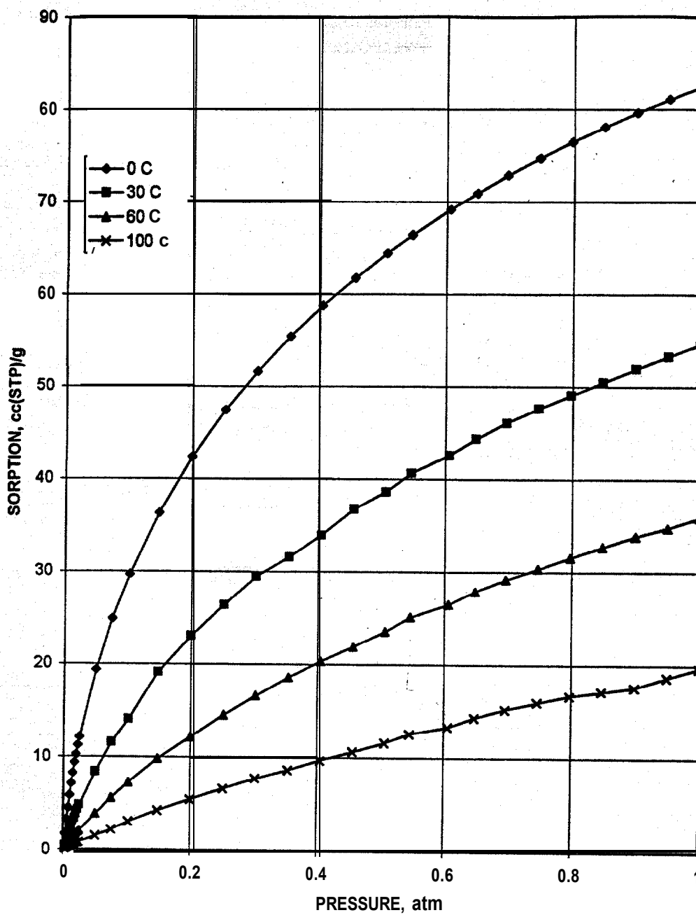
Figure 12. SORPTION OF CARBON DIOXIDE BY ACTIVATED CARBON FIBER. Monotonic increase of activity with increasing pressure is asymptotically diminished at increasing temperature.
