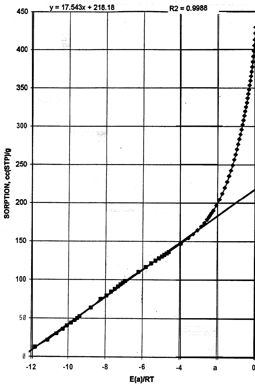
Figure 9. SORPTION OF NITROGEN BY ACTIVATED NMP RESIDUE A85 AT 77
