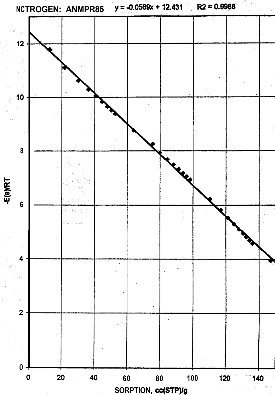
Figure 10. ENERGETIC RELATIONSHIPS FOR THE INITIAL UPTAKE OF NITROGEN BY ACTIVATED NMP RESIDUE A85 AT 77 K. Coordinate system changed to emphasize the energetic-s as dependent variable.
