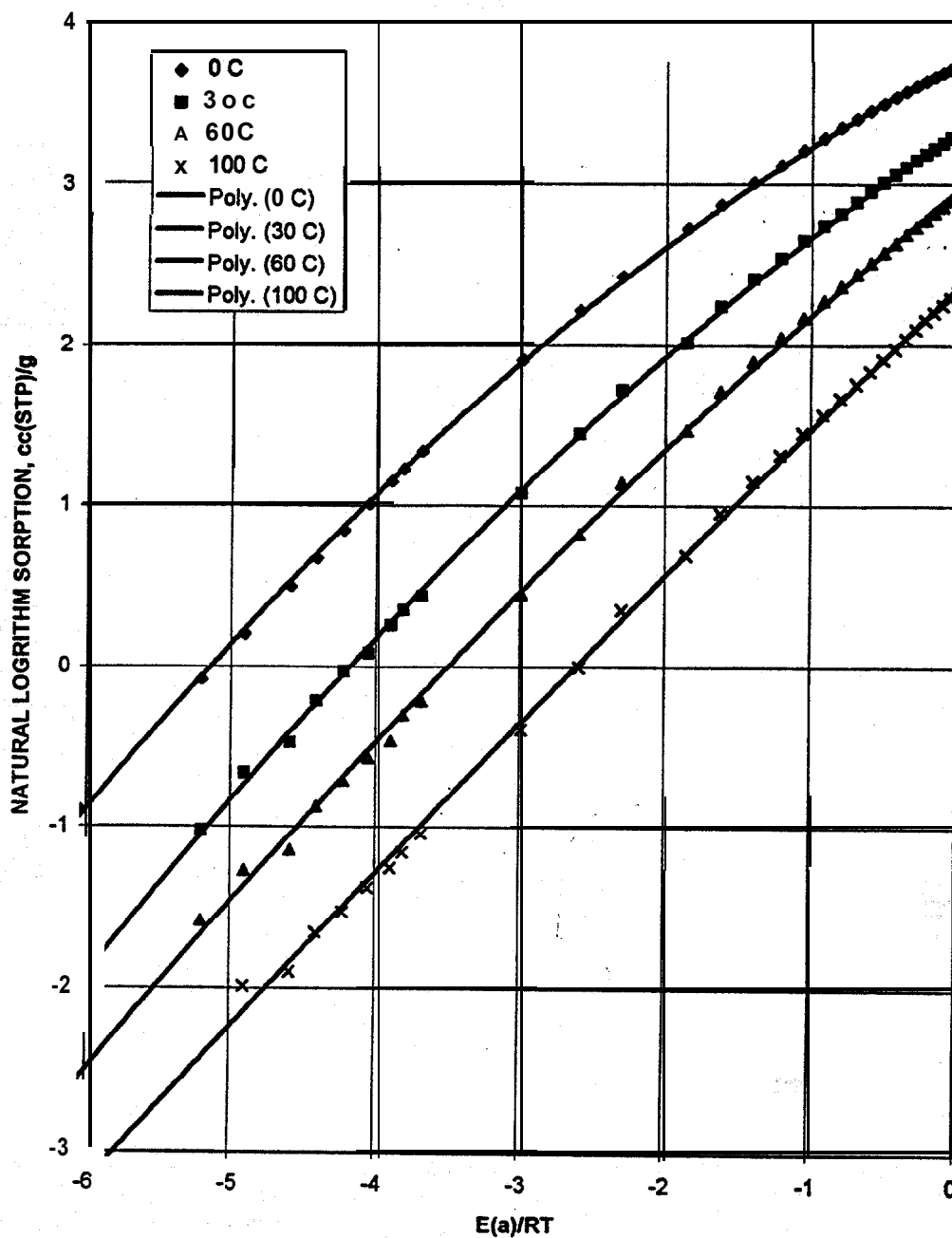
Figure 16. ENERGETICS OF METHANE SORPTION BY ACTIVATED CARBON FIBER.
