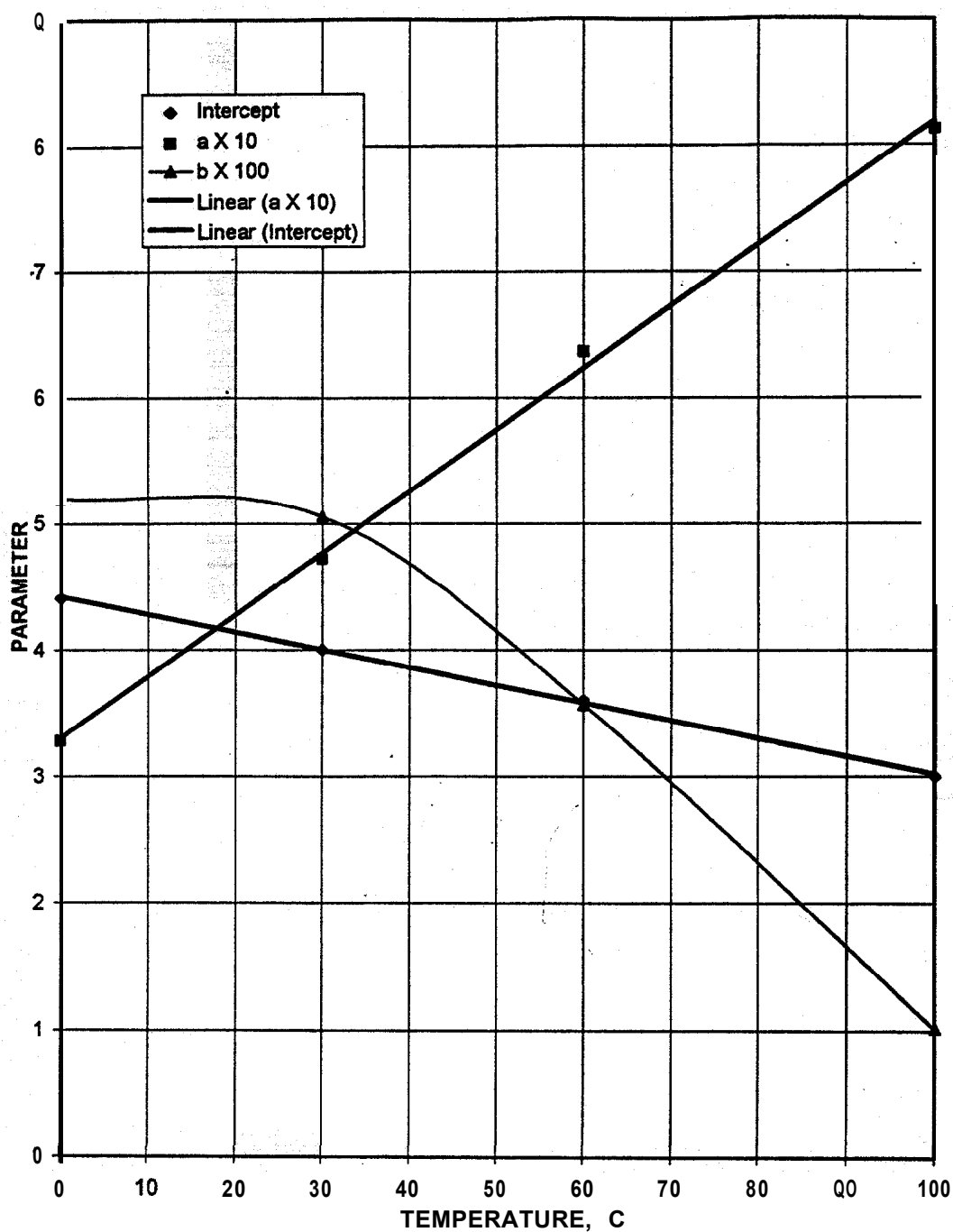
Figure 14. PARAMETER CORRELATION FOR CARBON DIOXIDE SORPTION BY ACTIVATED CARBON FIBER. Intercept and first order term vary linearly with temperature (regression lines). Second order term constant at lower temperatures (< ca. 30C).
