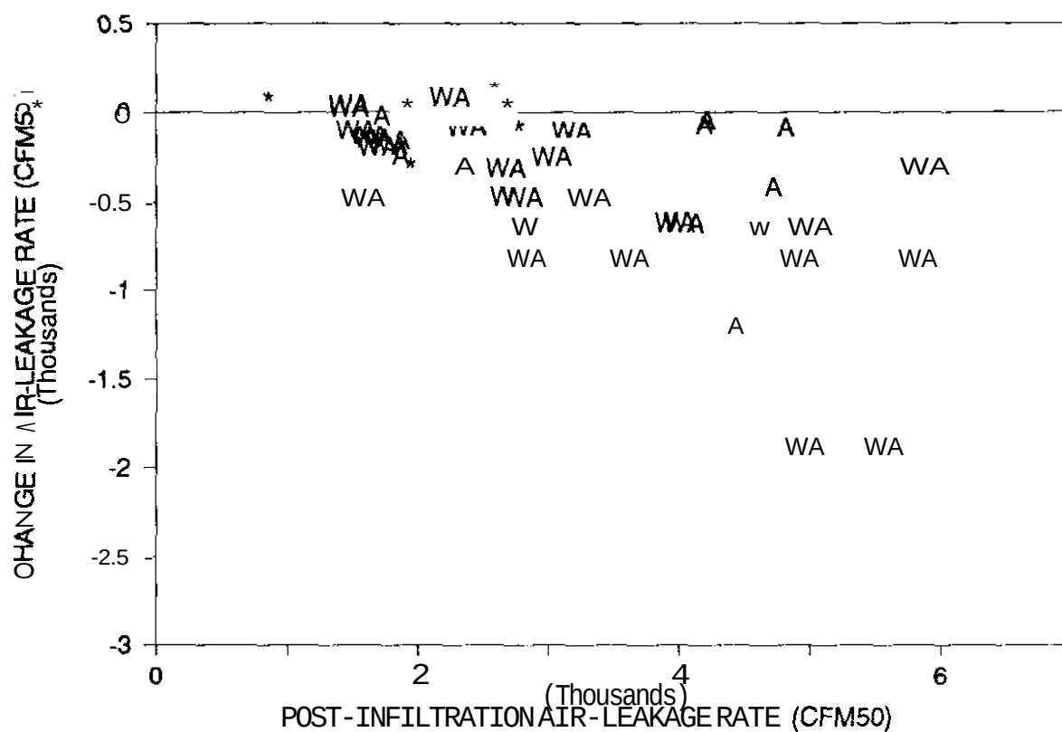
Fig. 7.2, Comparison of the change in air-leakage rate in the audit houses due to the installation of energy conservation measures other than infiltration reduction work to the air-leakage rate after infiltration reduction work was performed. An A indicates a house in which attic insulation with a predicted savings greater than 75 therms/year was installed, a W in which wall insulation with a predicted savings greater than this value was installed, a WA that both wall and attic insulation (each meeting this savings criterion individually) was installed, and a * that neither was installed.
