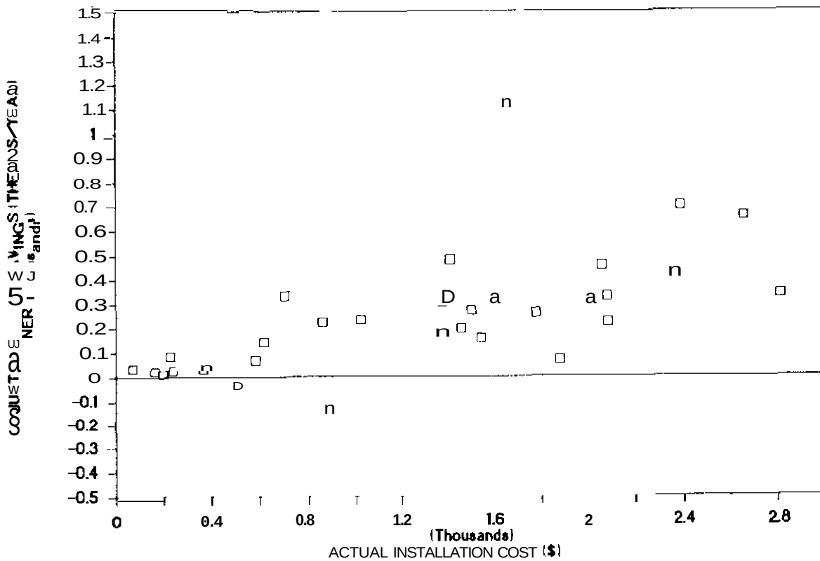
Fig. 9.3. Comparison of the adjusted space-heating energy savings of the audit houses to the actual cost for energy conservation measures designed to reduce space-heating energy consumption (excluding water-heating system measures) installed in the houses.
