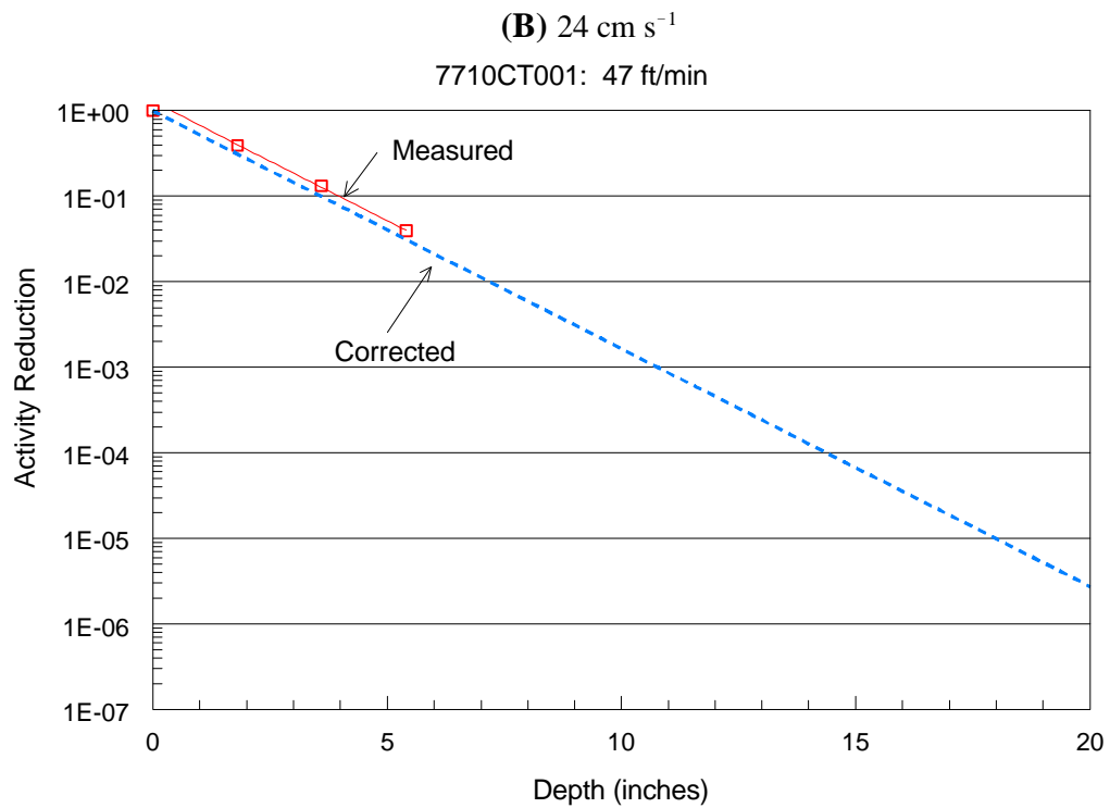
Fig. 4. Results for ^{220}\text{Rn} adsorption tests at low input concentrations with velocities of 18 \text{ cm s}^{-1} ( 35 \text{ ft min}^{-1} ) and 24 \text{ cm s}^{-1} ( 47 \text{ ft min}^{-1} ). The markers represent actual measurement data, the solid lines show a logarithmic fit to the measurement data, and the dashed lines (indicated as corrected ) show a line with a y-intercept of one and a slope equal to that of the logarithmic fit.
