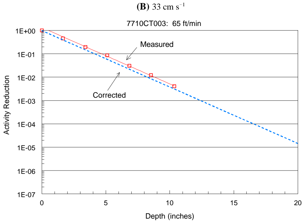
Fig. 5. Results for ^{220}\text{Rn} adsorption tests at low input concentrations with velocities of 10 and 33 \text{ cm s}^{-1} ( 20 and 65 \text{ ft min}^{-1} ). The markers represent actual measurement data, the solid lines show logarithmic fits to the measurement data, and the dashed lines (indicated as corrected ) show lines with a y-intercept of one and a slope equal to that of the logarithmic fit.
