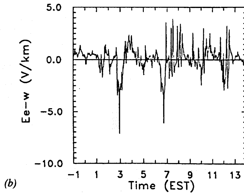
Fig. 5.2. Computed electric fields for measured fields in Fig. 3.1 with \sigma=1.0 \times 10^{-4} mhos/meter. (a) North-south field, (b) east-west field.
