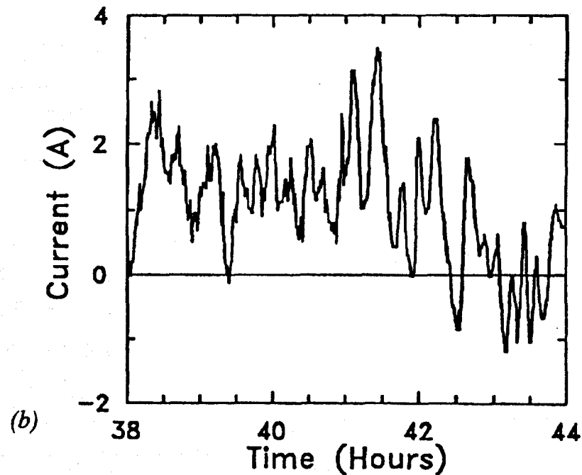
Fig. 3.3. Neutral current measured at the Missouri Ave. 6.9-kV/12-kV substation starting on April 4, 1990. (a) GIC Measured over a 100-h period, (b) GIC measured over a 6-h period. Source: C.K. Bush, Atlantic Electric Co.
