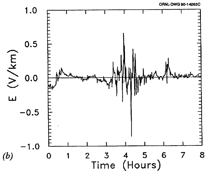
Fig. 3.5. Geomagnetic and electric fields at Hydro-Québec's Boucherville substation on July 13, 1982. (a) Measured north-south geomagnetic field disturbance, (b) computed east-west electric field for a ground resistivity of 55.6 \Omega\text{-m} .
