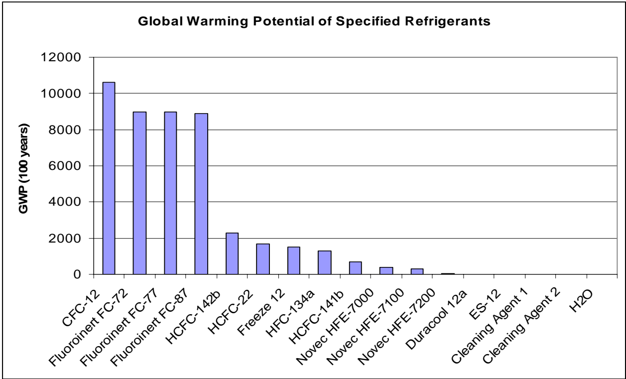
Fig. 2. Refrigerant GWP.
