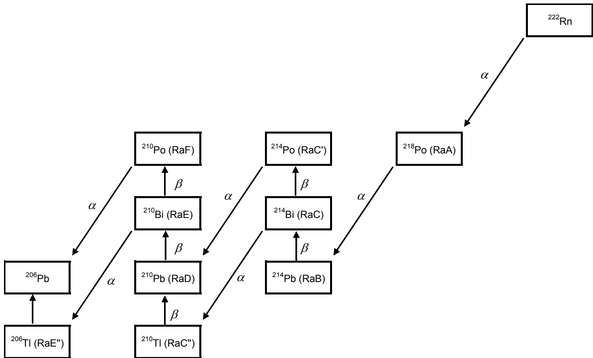
Fig. 1. Major decay mode of ^{222}\text{Rn} and its daughters.
