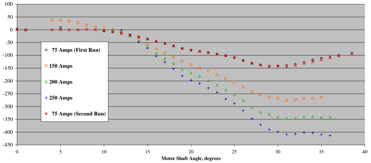
Fig. 3.4. Motor shaft angle versus torque (rotor locked).
