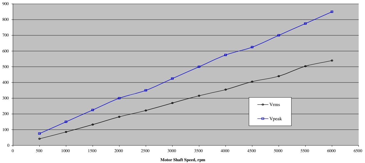
Fig. 3.6. Motor back-emf voltage versus motor shaft speed.
