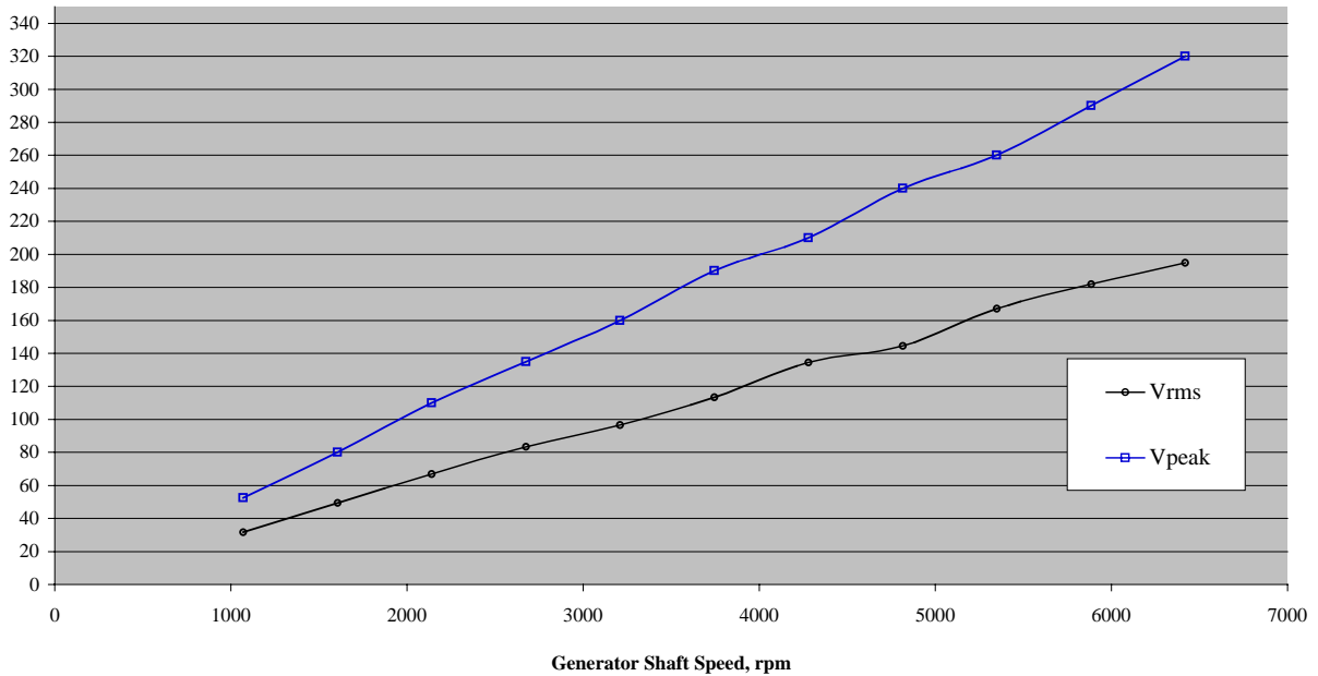
Fig. 3.7. Generator back-emf voltage versus generator shaft speed.
