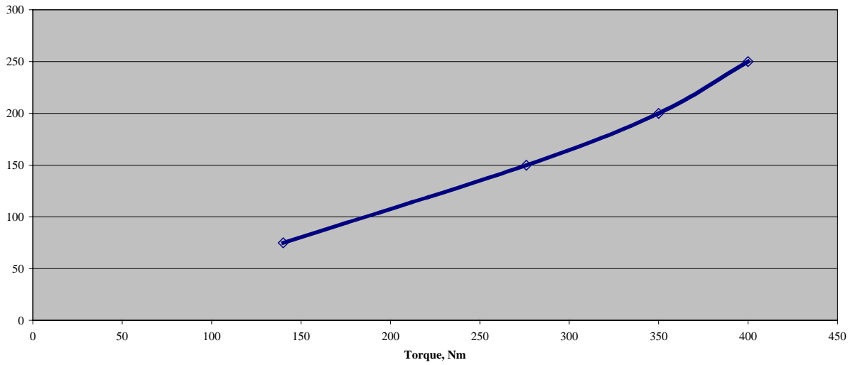
Fig. 3.5. Locked rotor peak torque as a function of current.
