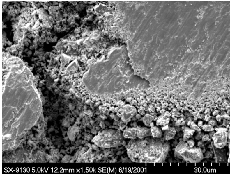
Fig. 8. Compressed debris layer formed from a 600° C test on 304 stainless steel.
