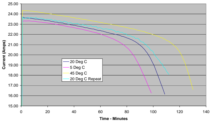
60Ah Battery Discharge Waveforms
