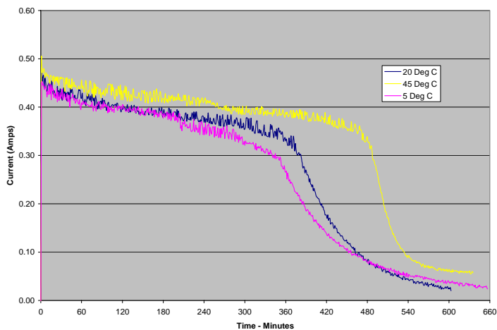
3.4 Ah Battery Charge Current
