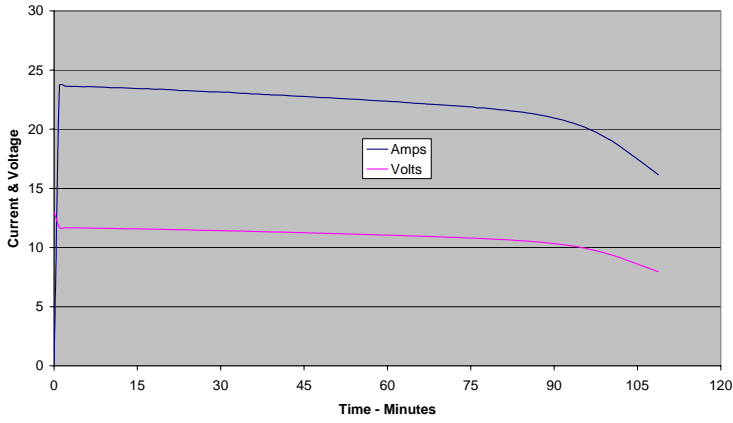
60Ah Battery Discharge at 20C
