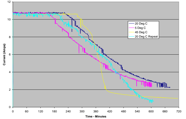
110Ah Battery Charge Waveforms
