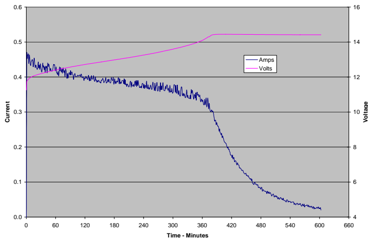
3.4 Ah Battery Charge at 20C
