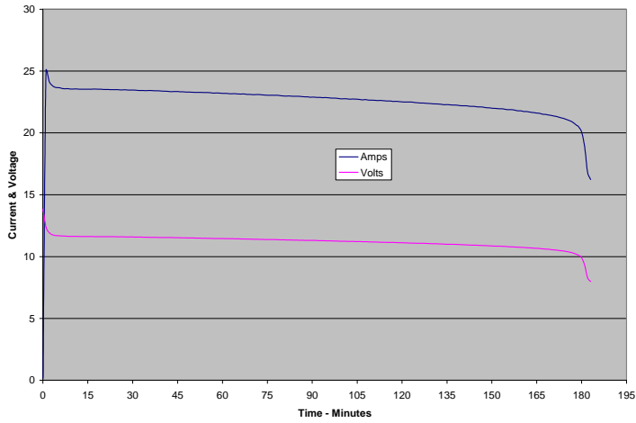
110Ah Battery Discharge at 20C
