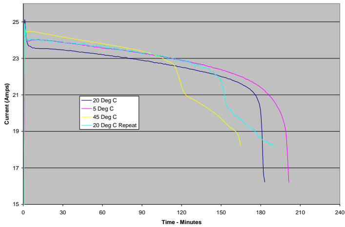
110Ah Battery Discharge Waveforms
