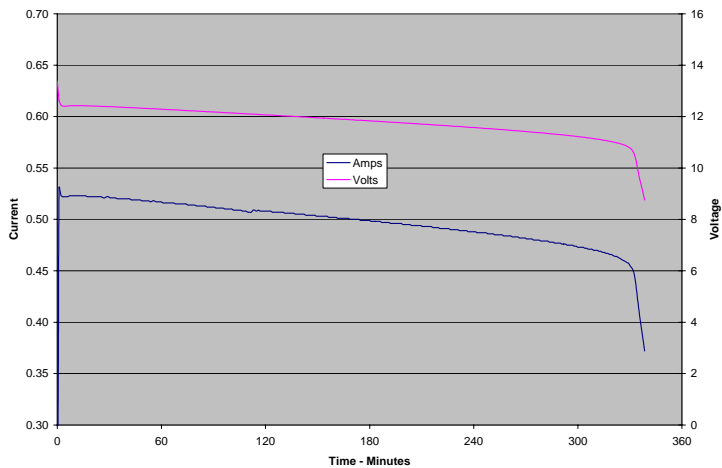
3.4 Ah Battery Discharge at 20C
