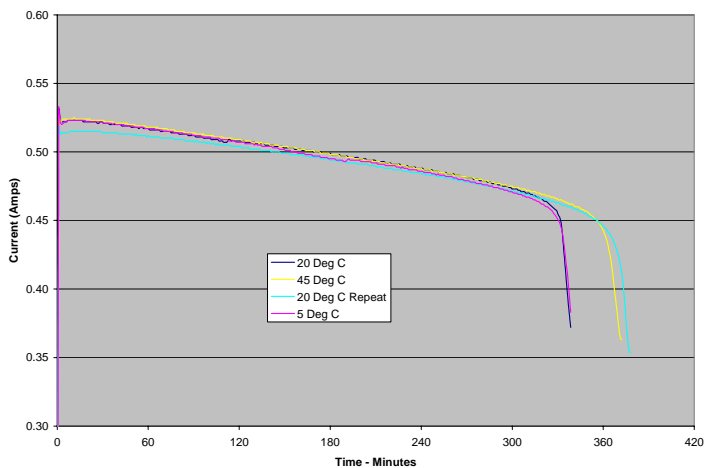
3.4 Ah Battery Discharge Current
