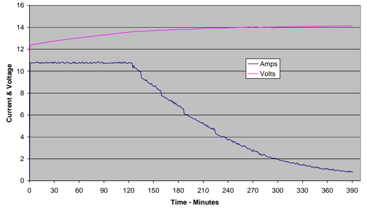
60Ah Battery Charge at 20C
