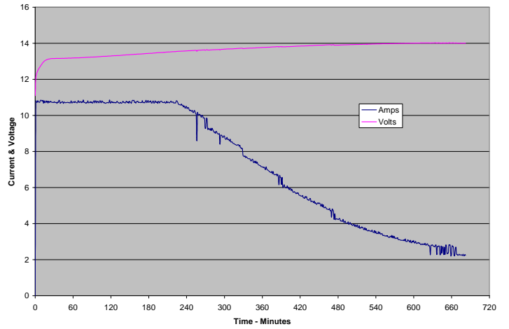
110Ah Battery Charge at 20C
