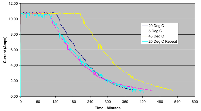
60Ah Battery Charge Waveforms
