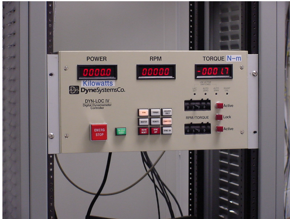
Fig. 3. Dynamometer controller display panel.
