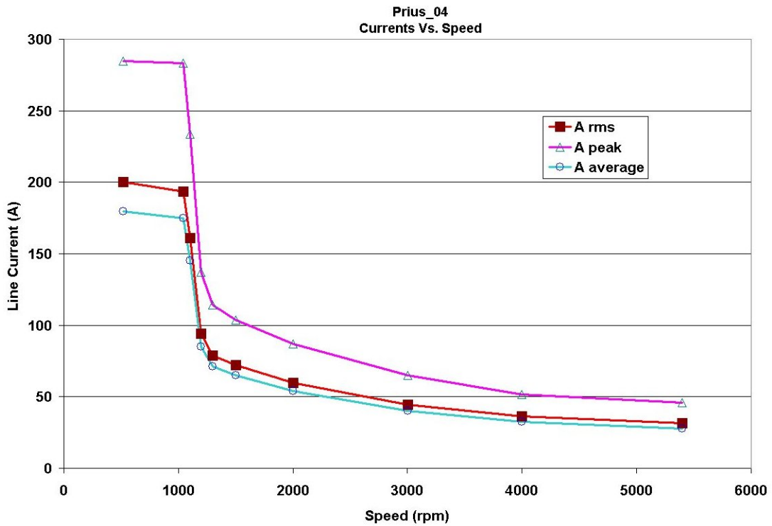
Fig. 5.4. Stator current vs. machine speed for the full-size IPM.
