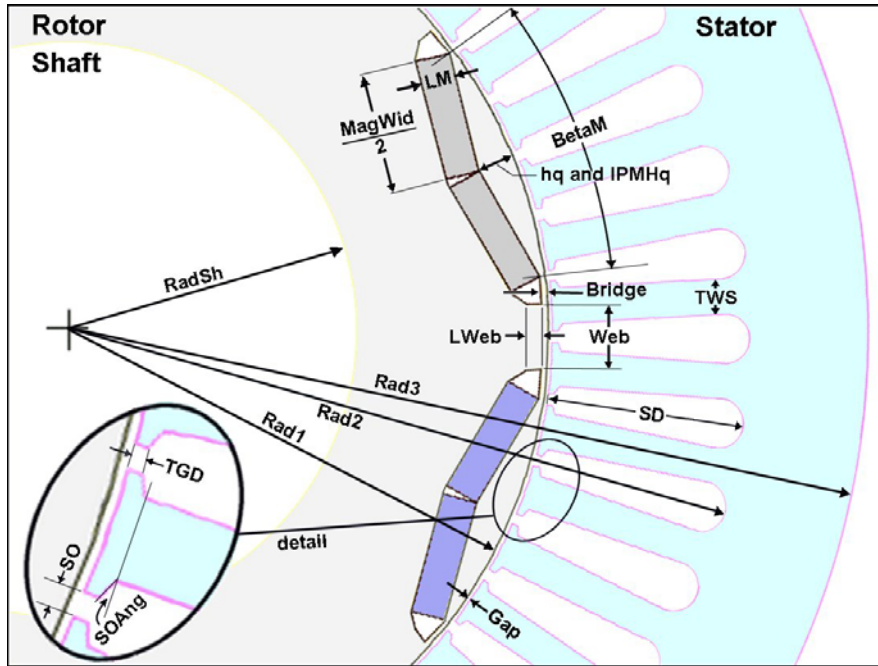
Fig. 5.2. IPM machine sketch with critical dimensions.
