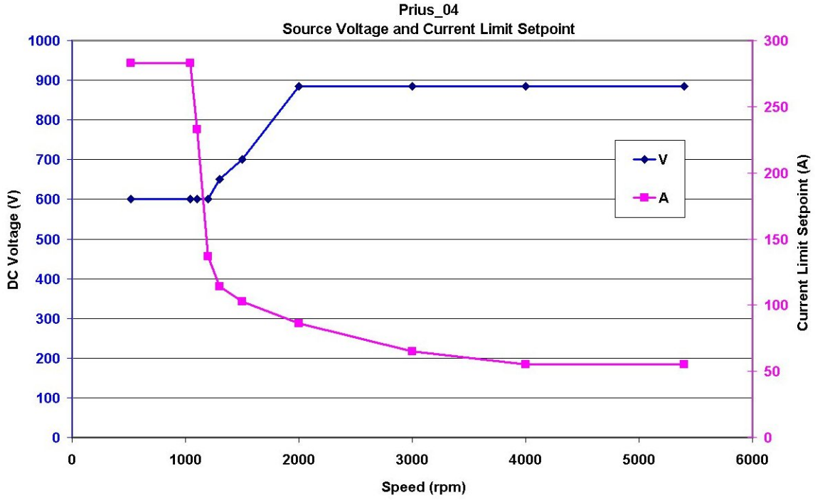
Fig. 5.5. Source voltage and ISP vs. machine speed for the full-size IPM.
