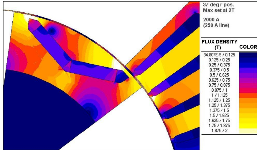
Fig. 5.10. Flux density color-coded map of rotor sector and portion of stator with a 2 Tesla ceiling.
