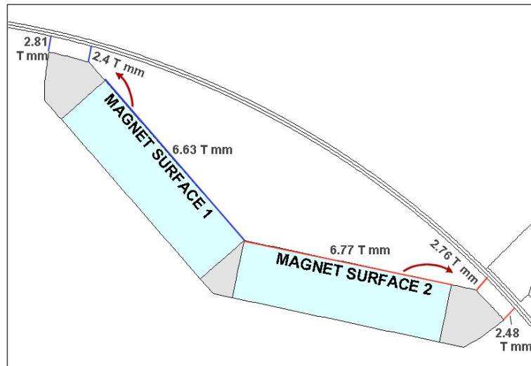
Fig. 5.12. Results of FEA analysis to determine the fraction of magnetic flux strength that is lost across the narrow bridge paths.
