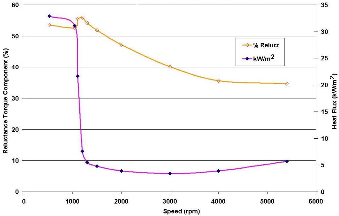
Fig. 5.6. Reluctance torque and heat flux vs. speed for the full-size IPM.
