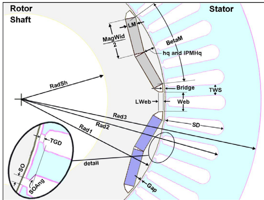
Fig. D.1. Physical parameters used in the SPEEDCAD model (IPM machine).
