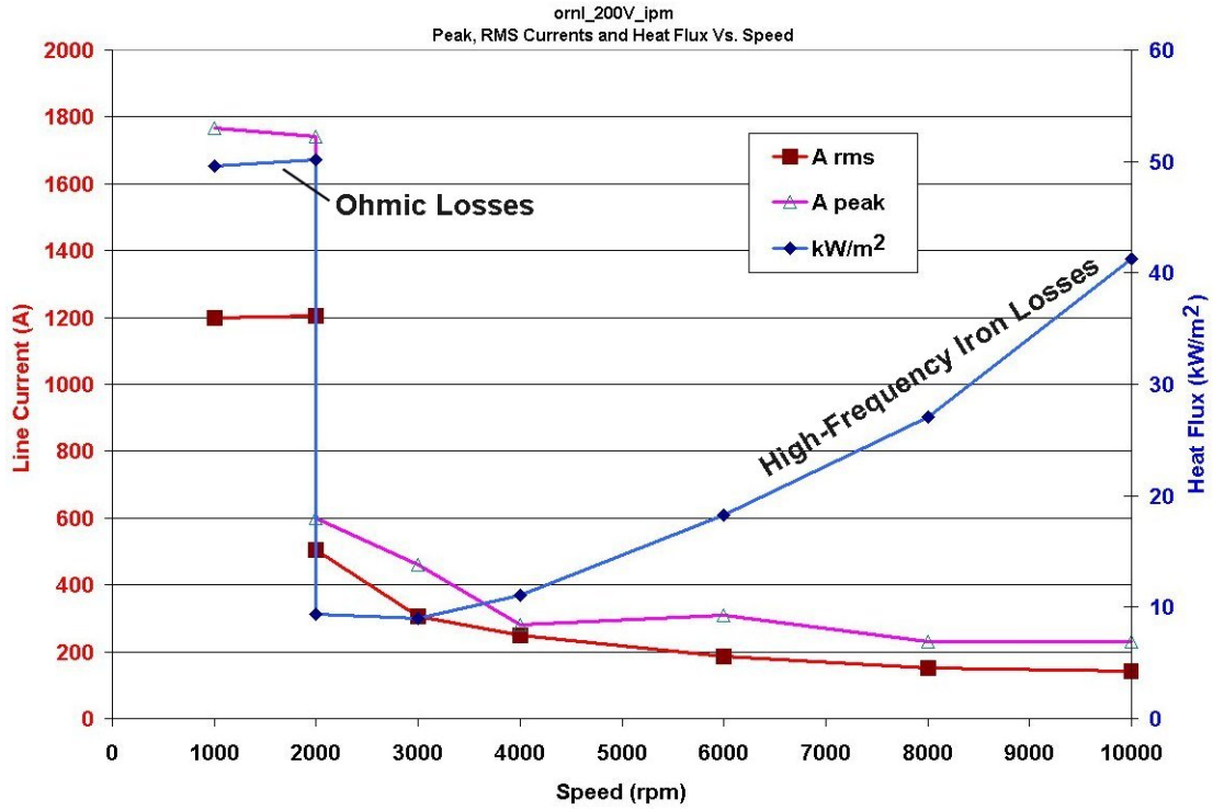
Fig. 5.15. Line current and heat flux for high-speed IPM machine.
