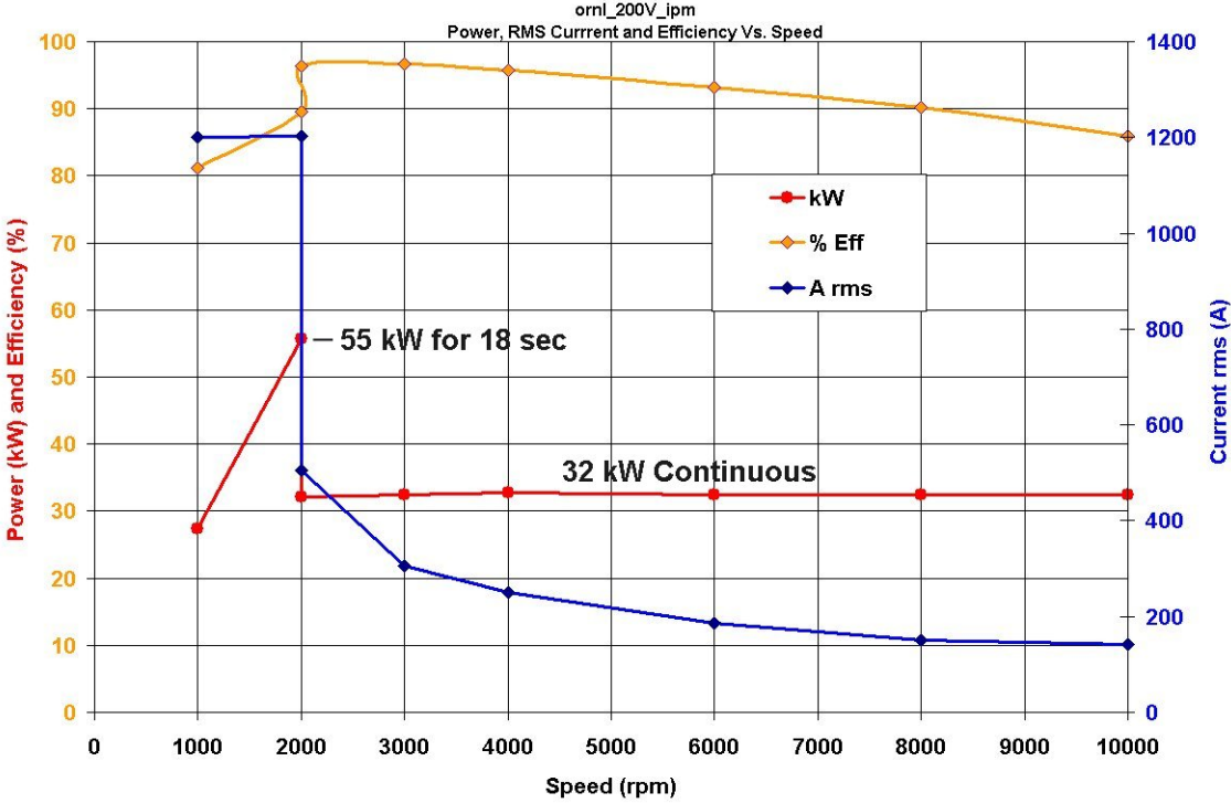
Fig. 5.13. Power, efficiency, and current vs. speed for high-speed IPM machine.
