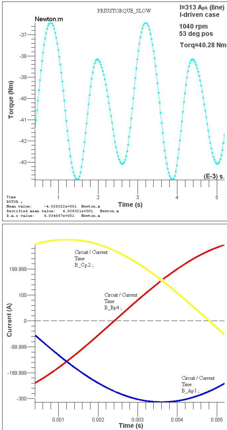
Fig. 5.8. Torque and stator current over time with baseline machine operating at 1040 rpm.
