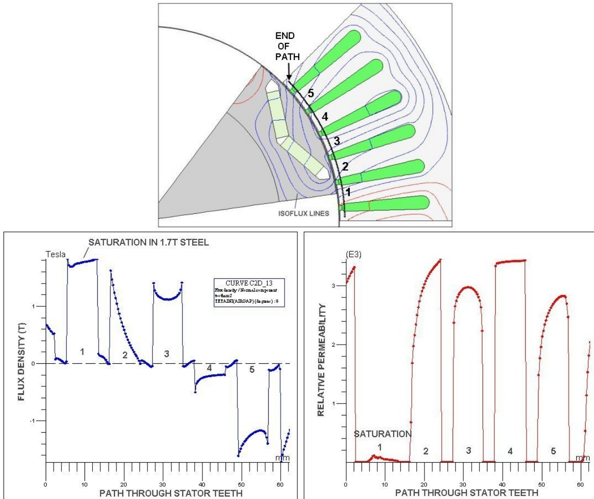
Fig. 5.11. Flux density and relative permeability over a pre-defined path across stator teeth.
