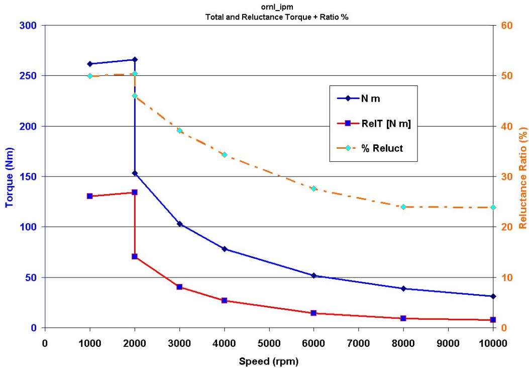
Fig. 5.14. Torque, reluctance torque, and torque ratio for high-speed IPM machine.
