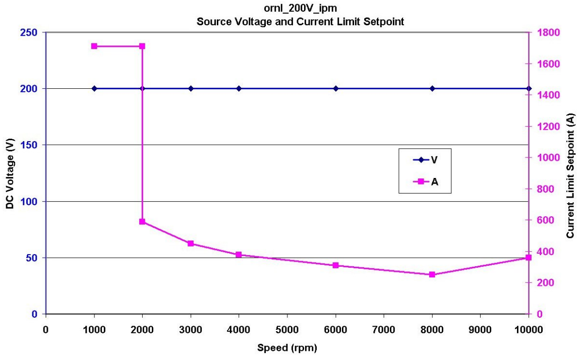
Fig. 5.16. Vdc and line ISP for high-speed IPM machine.
