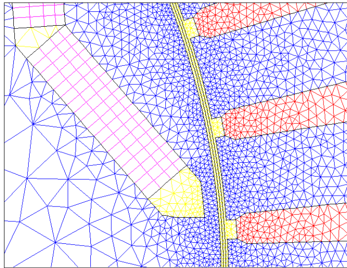
Fig. 5.7. Mesh of elements reflecting an emphasis on precision at critical machine areas.
