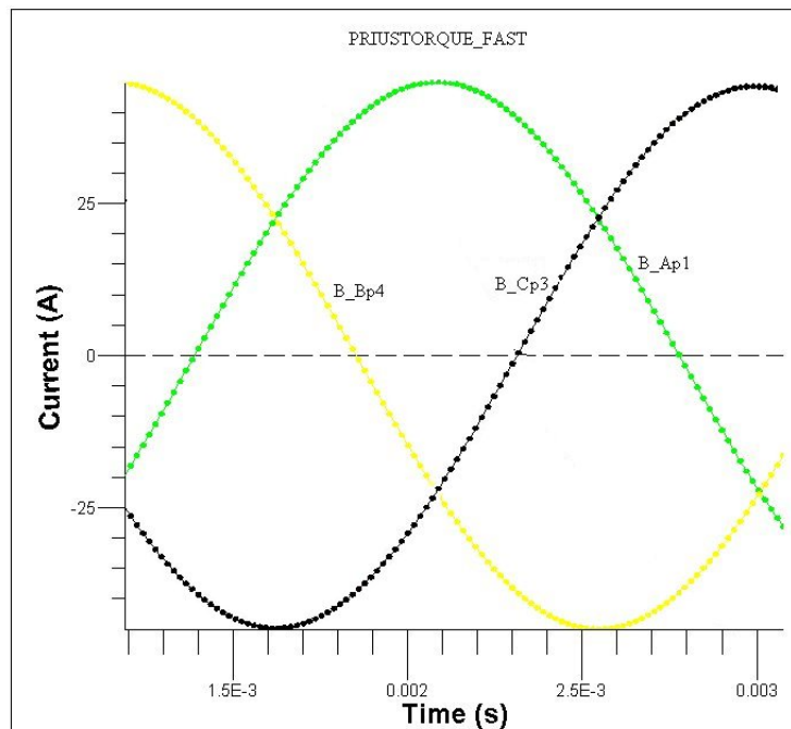
Fig. 5.9. Torque and stator current over time with baseline machine operating at 5400 rpm.
