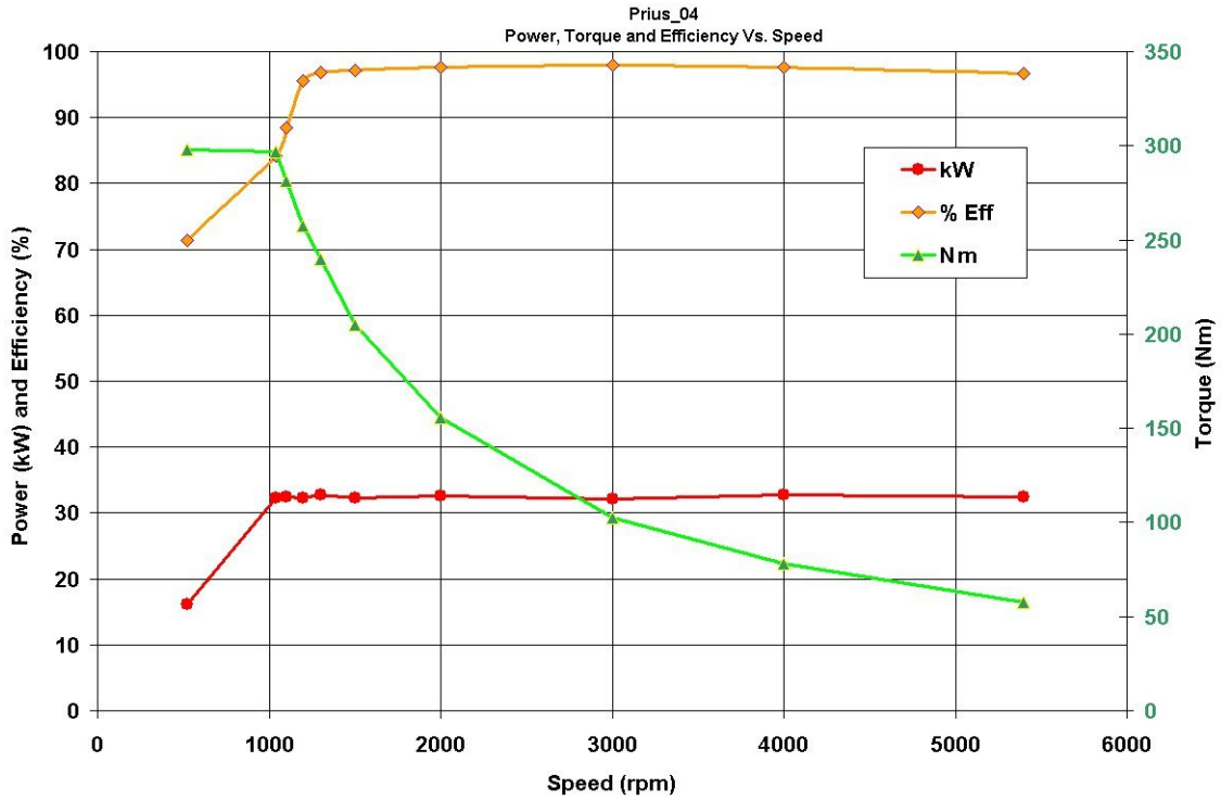
Fig. 5.3. Power, efficiency, and torque vs. machine speed for the full-size IPM.
