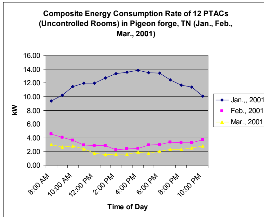
Fig. 10. Graph of electric demand for heating versus time of day for January, February and March 2001 for 12 uncontrolled rooms.
