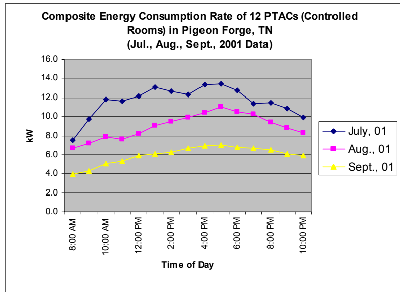
Fig. 7. Graph of electric demand for cooling versus time of day for July, August and September 2001 for 12 controlled rooms.
