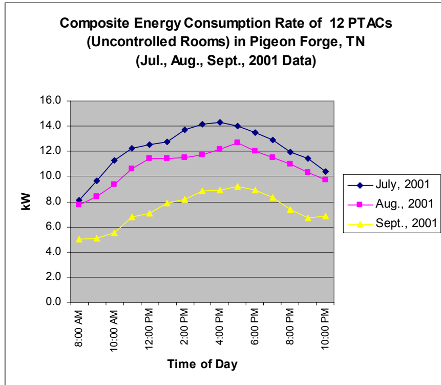
Fig. 8. Graph of electric demand for cooling versus time of day for July, August and September 2001 for 12 uncontrolled rooms.
