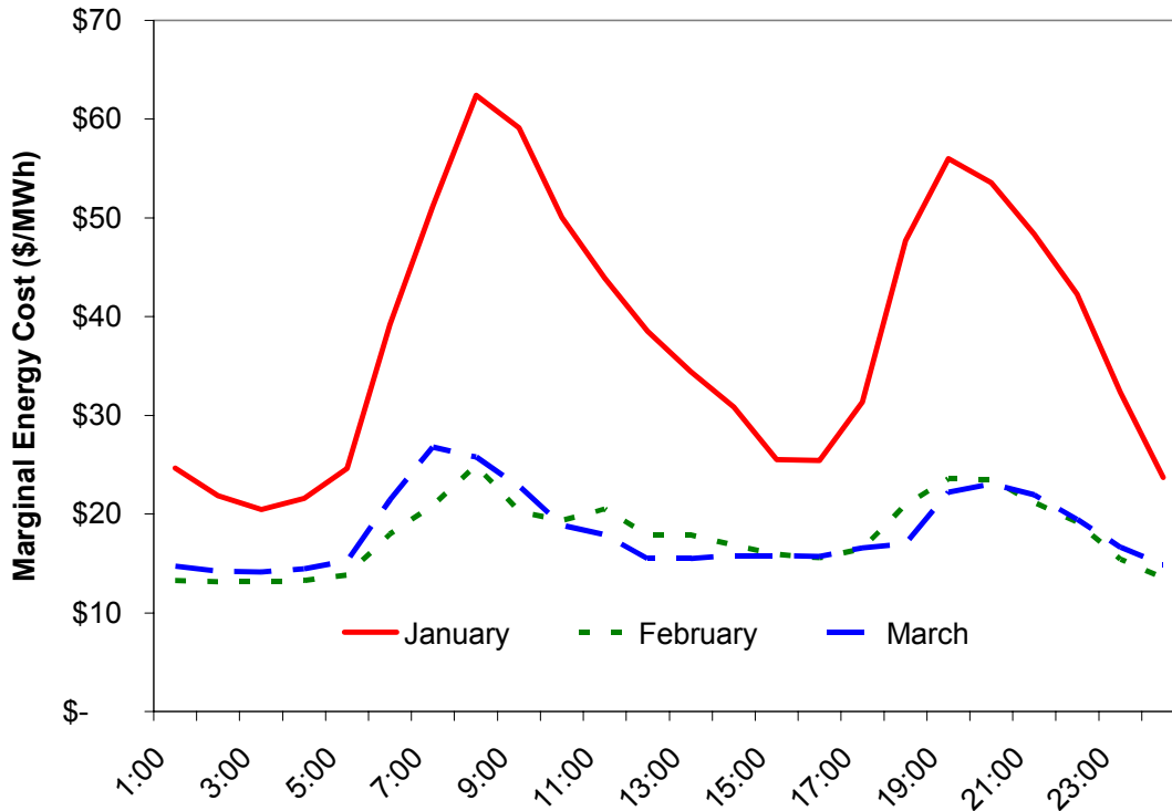
Fig. 14. TVA average hourly system winter 2001 marginal energy cost.
