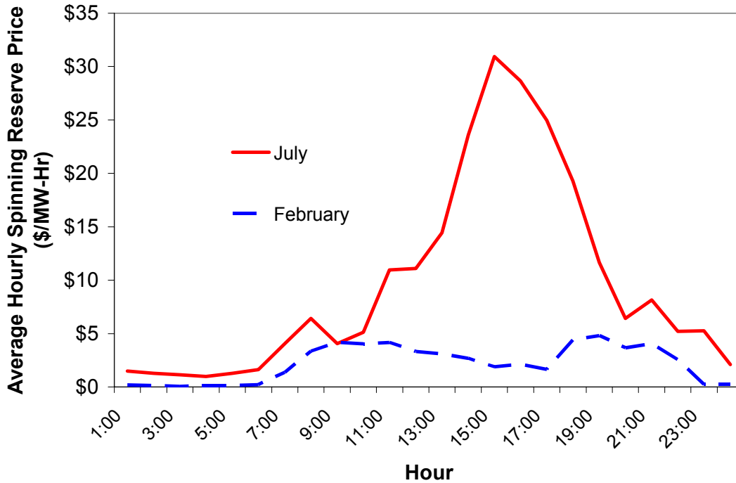
Fig. 15. Average hourly CAISO spinning reserve prices for July and February 2002.
