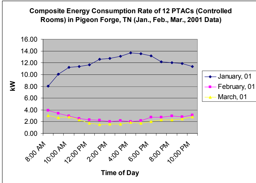
Fig. 9. Graph of electric demand for heating versus time of day for January, February and March 2001 for 12 controlled rooms.
