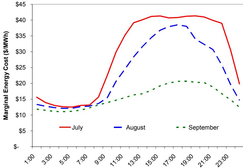
Fig. 12. TVA average hourly system summer 2001 marginal energy cost.
