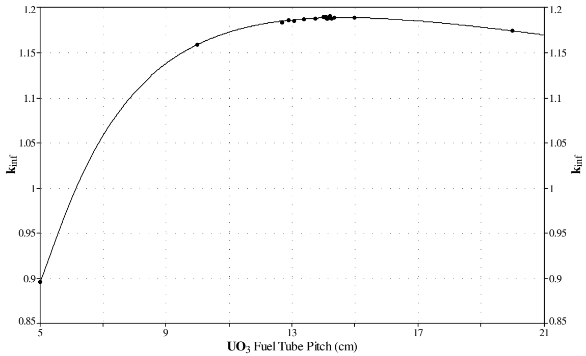
Fig. 4.1. Variation of k_{inf} with UO 3 fuel tube pitch.
