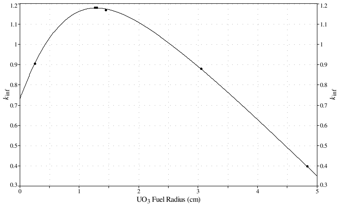
Fig. 4.2. Variation of k_{inf} with UO 3 fuel radius.
