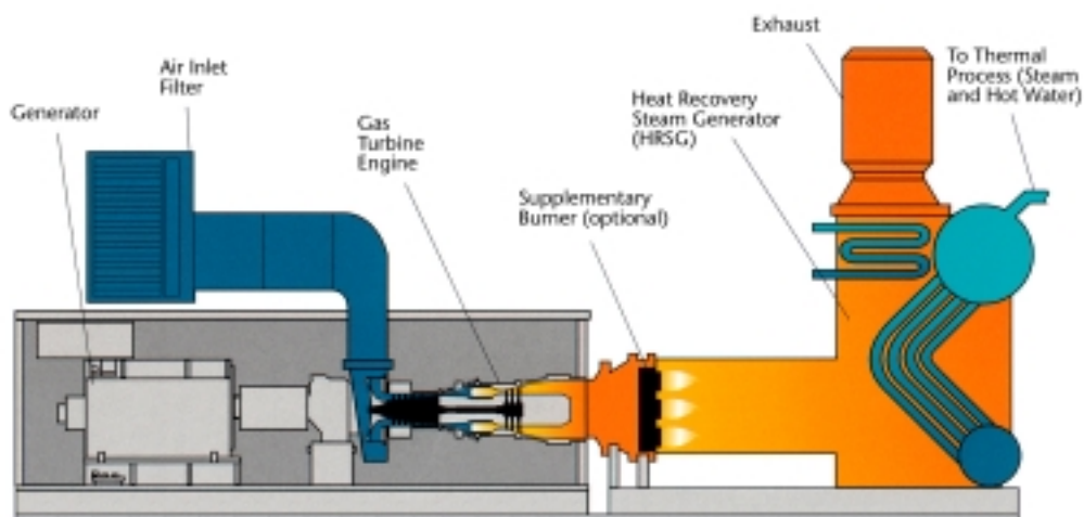
Fig. 2. Components of typical gas-fired turbine CHP unit.
