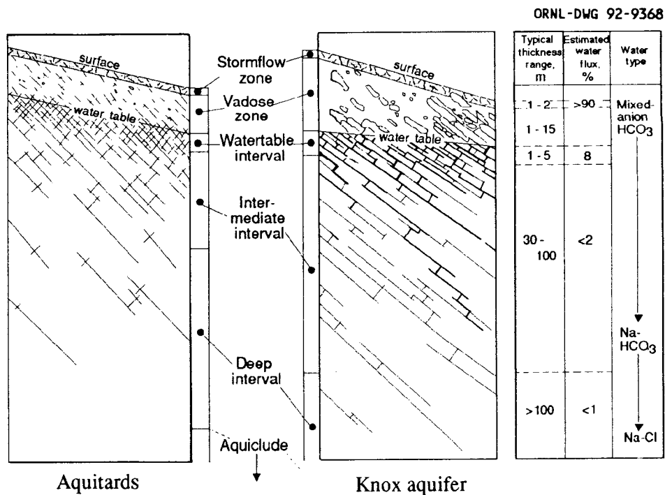
Not to scale Fig. 2.1. Schematic vertical relationships of flow zones of the ORR, estimated thicknesses, water flux, and water types.
