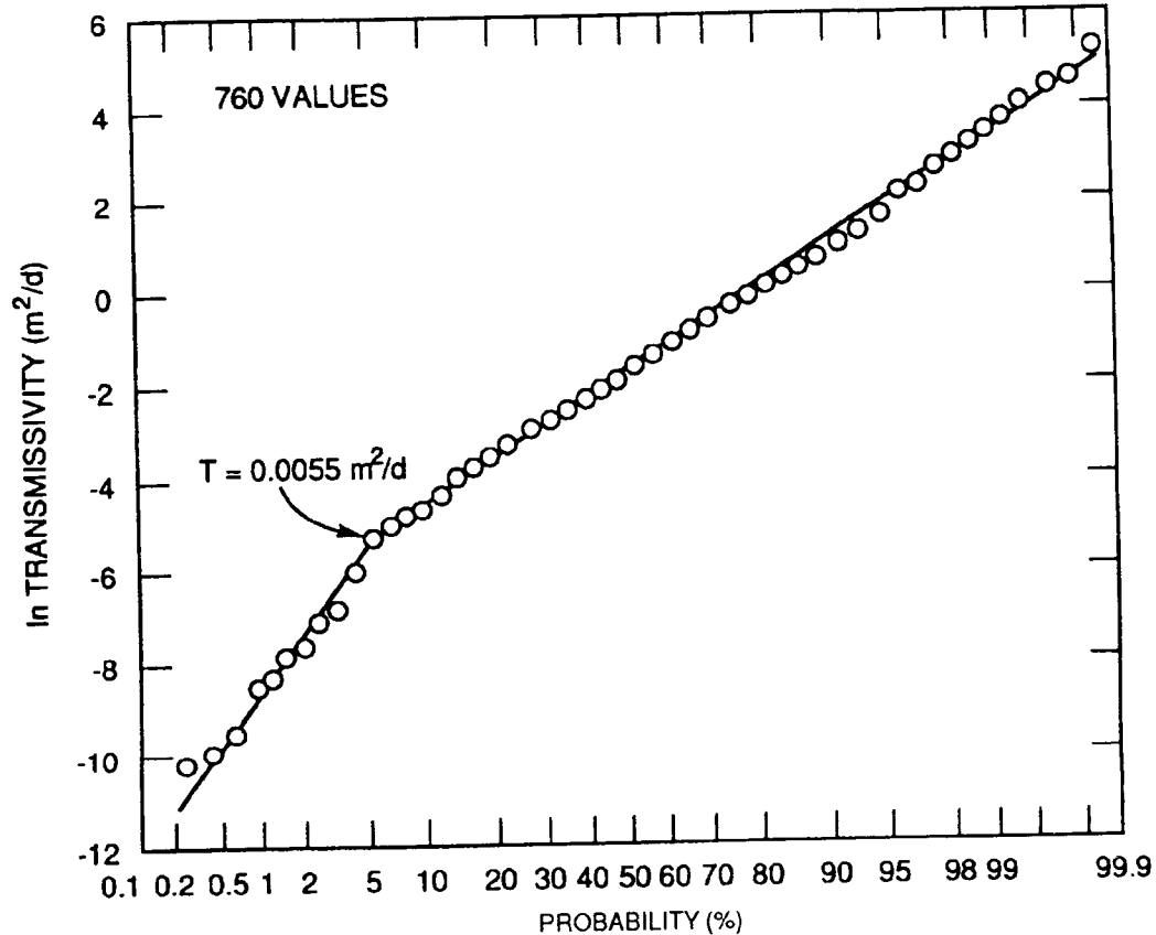
Fig. 3.9. A cumulative probability graph of transmissivity data shows two lognormal populations.
