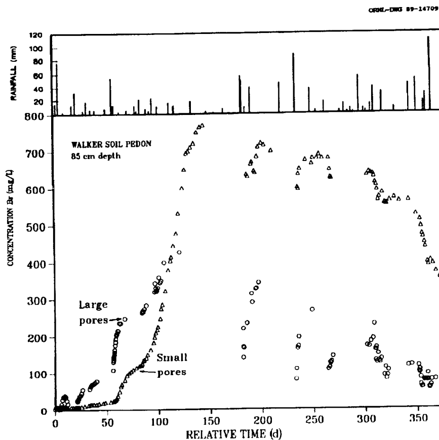
Fig. 3.7. Br^- concentration observed at a depth of 85 cm as a function of time.
