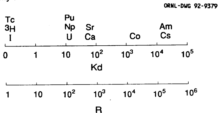
Fig. 3.13. Approximate order of magnitude of laboratory-measured sorption coefficients (Kd) and calculated retardation factors (R) for selected radionuclides and calcium and soil and rock materials of the ORR. A ratio of bulk density to porosity of 10 was assumed for computing R.
