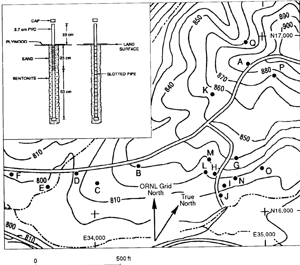
Fig. 3.3. Locations of stormflow monitoring tubes in the study area in headwaters of Melton Branch. Inset shows design of monitoring tubes for collection of water samples (left) and monitoring of water levels (right).
