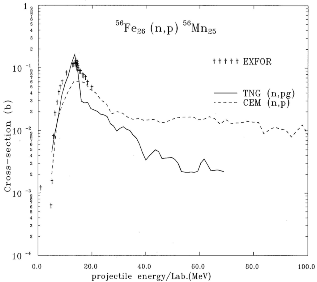
Figure 956-Fe (n,p) cross section. There is a discontinuity in the curvatures of the calculated data of CEM95 and TNG above 30 MeV. Both calculations give similar results in the 5 to 30 MeV region where the CEM95 results are better than the TNG results.
