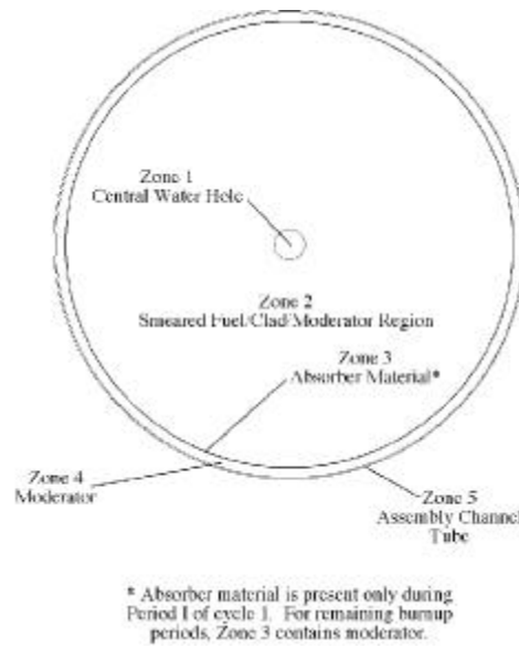
Fig. 2. One-dimensional assembly approximation for Trino Vercelles assemblies.
