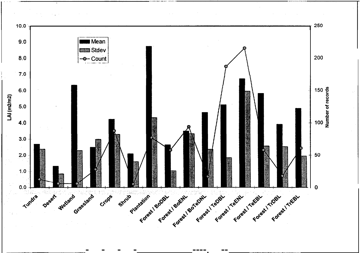
Fig. 2. Distribution of approximately 1000 historical estimates of LAI, summarized by biome/cover type. See Table 1(b) for explanation of abbreviated biome names.
