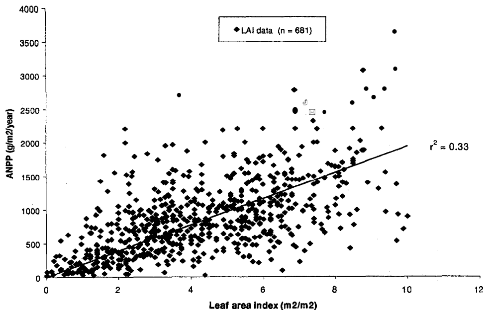
Fig. 5. ANPP as a function of LAI for a subset of the data for which both parameters were available.
