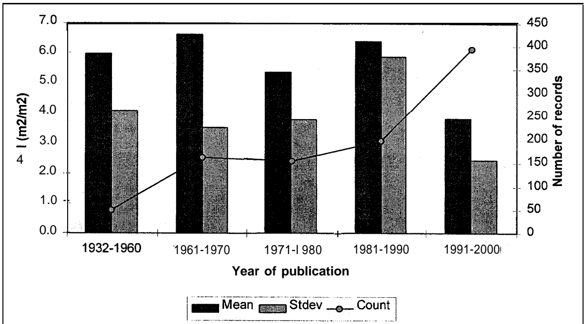
Fig. 3. Distribution of reported LAI values, classified by decade of publication,
