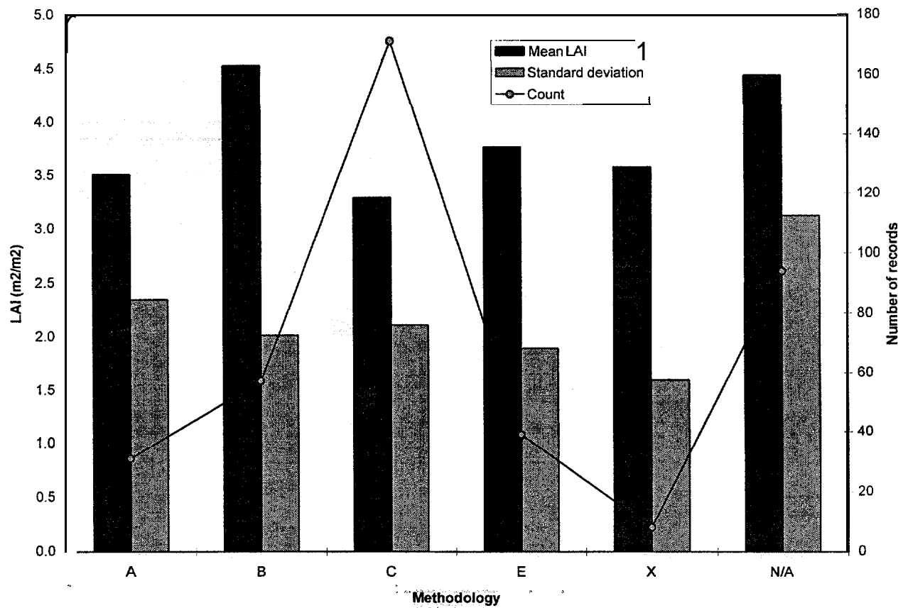
Fig. 4. Distribution of LAI data published in the decade 1991-2000, plotted by estimation methodology. Where a combination of methods was used, only the principal method is tallied. A, Destructive harvest; B, Litterfall; C, Allometry; E, Indirect noncontact (LAI-2000 or other); X, Unknown (i.e., literature was checked and method was not specified); N/A, Not available (i.e., literature was not available for checking).
