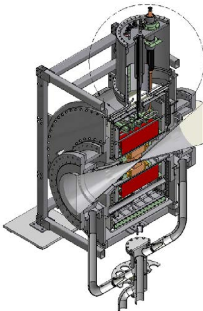
Figure 1. Cross section of the HZB hybrid magnet from Ref [4]. The bore of the magnet is along the same direction as the incident neutron beam. SC coils are shown in red surrounding the inner resistive coils shown in orange.
