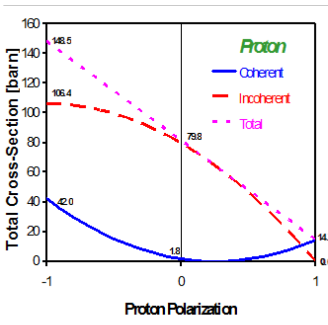
Figure 5. Coherent, incoherent and total scattering cross section of hydrogen as a function of the proton polarization for fully polarized neutrons. 9 Figure is inspired by Fig. 1 of Ref. [10].
