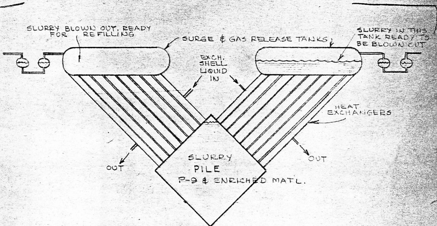
WIGNER "PULSATING" PILE
