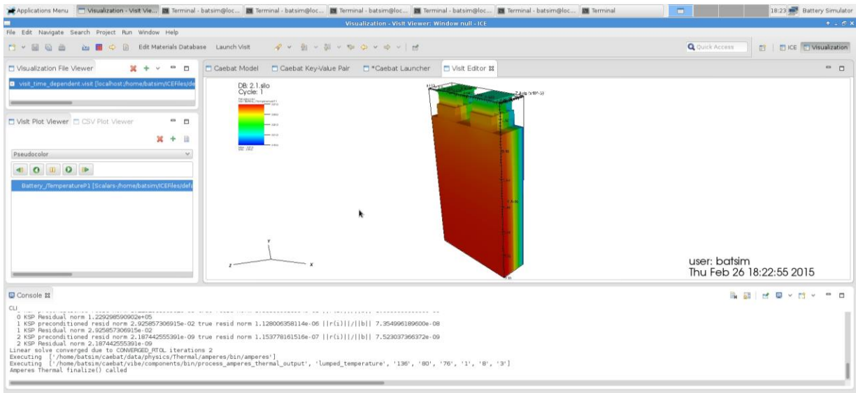
Fig. 29. Temperature distribution in 4P Li-ion module
