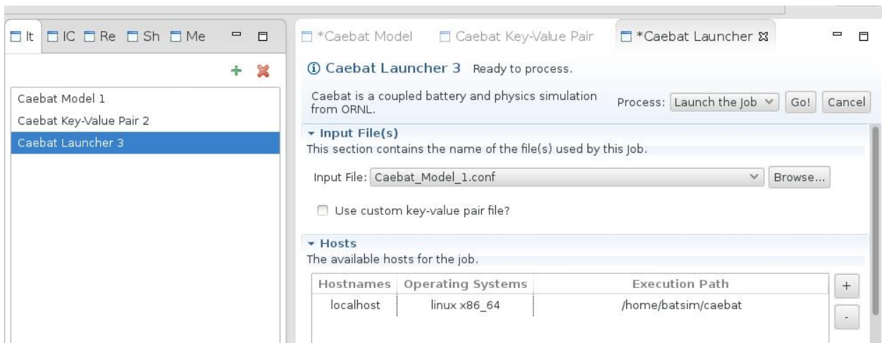
Fig. 23. Battery simulation launcher in ICE
