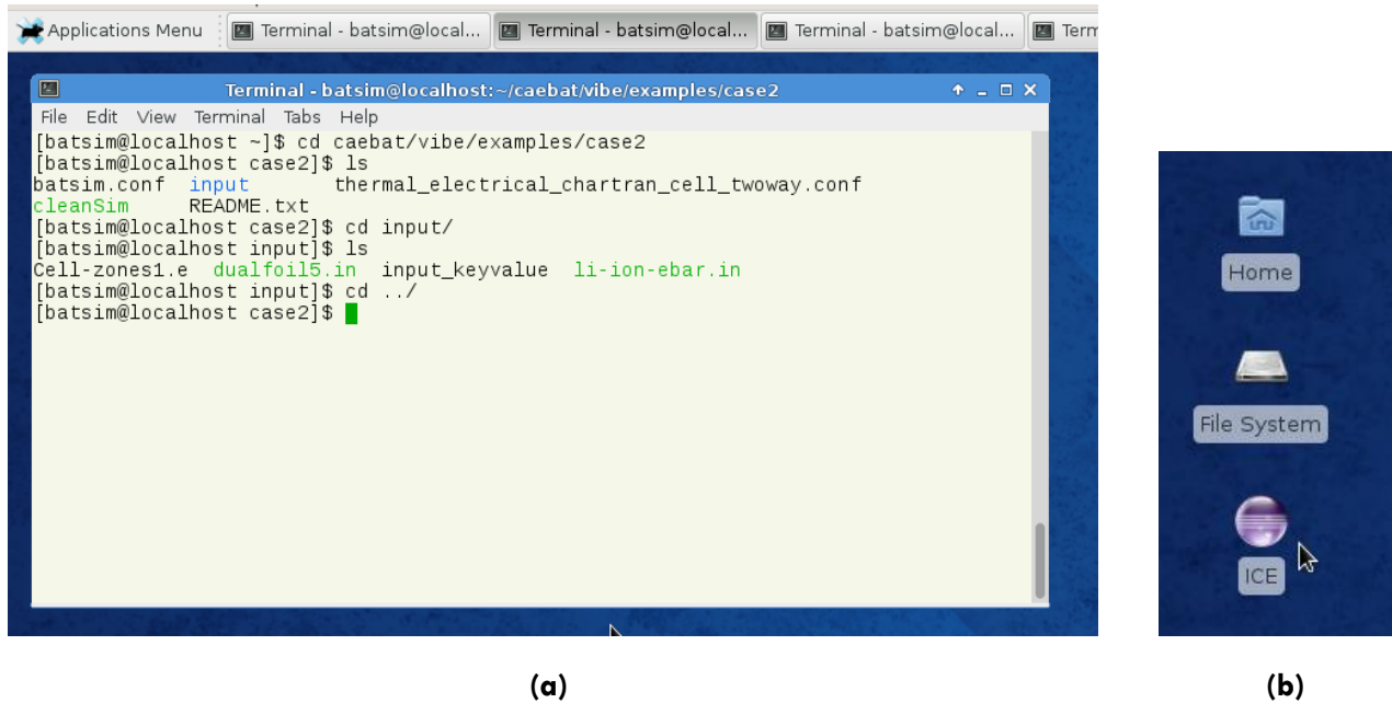
Fig. 17. Using command line (a) or ICE (b) to setup and run a simulation in VIBE
