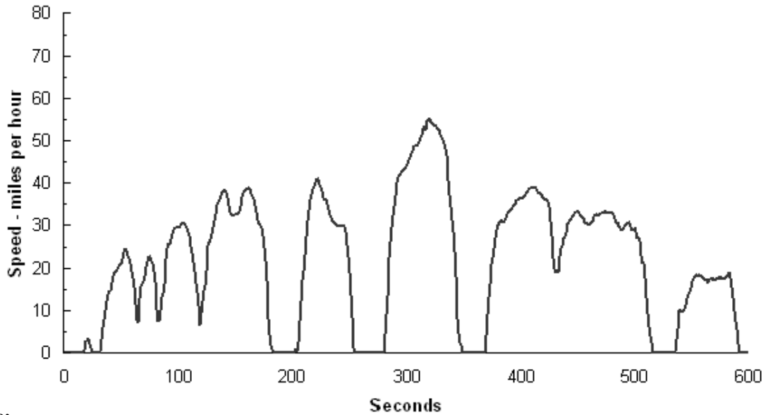
Figure 4.5. Air Conditioning Driving Cycle
