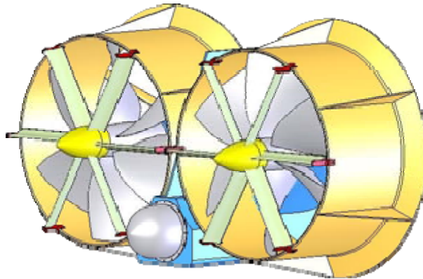
Figure 3. Artist's conception of a UEK Corporation's dual hydroturbine unit, a ducted, horizontal axis hydrokinetic turbine. Source: UEK Corporation http://www.uekus.com/index.html
