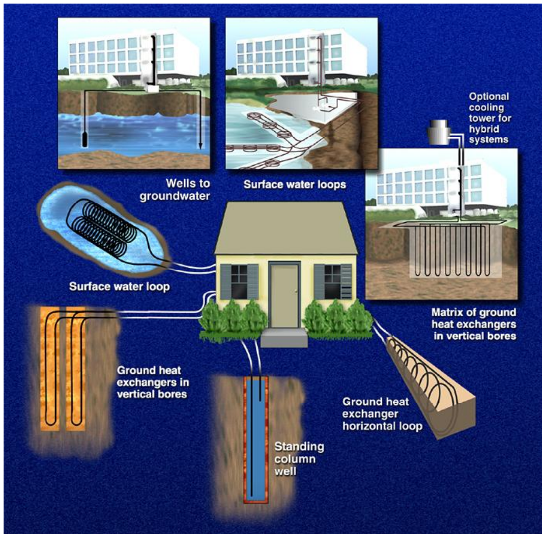
Fig. 1 Typical options for ground heat exchanger used in GHP systems.
