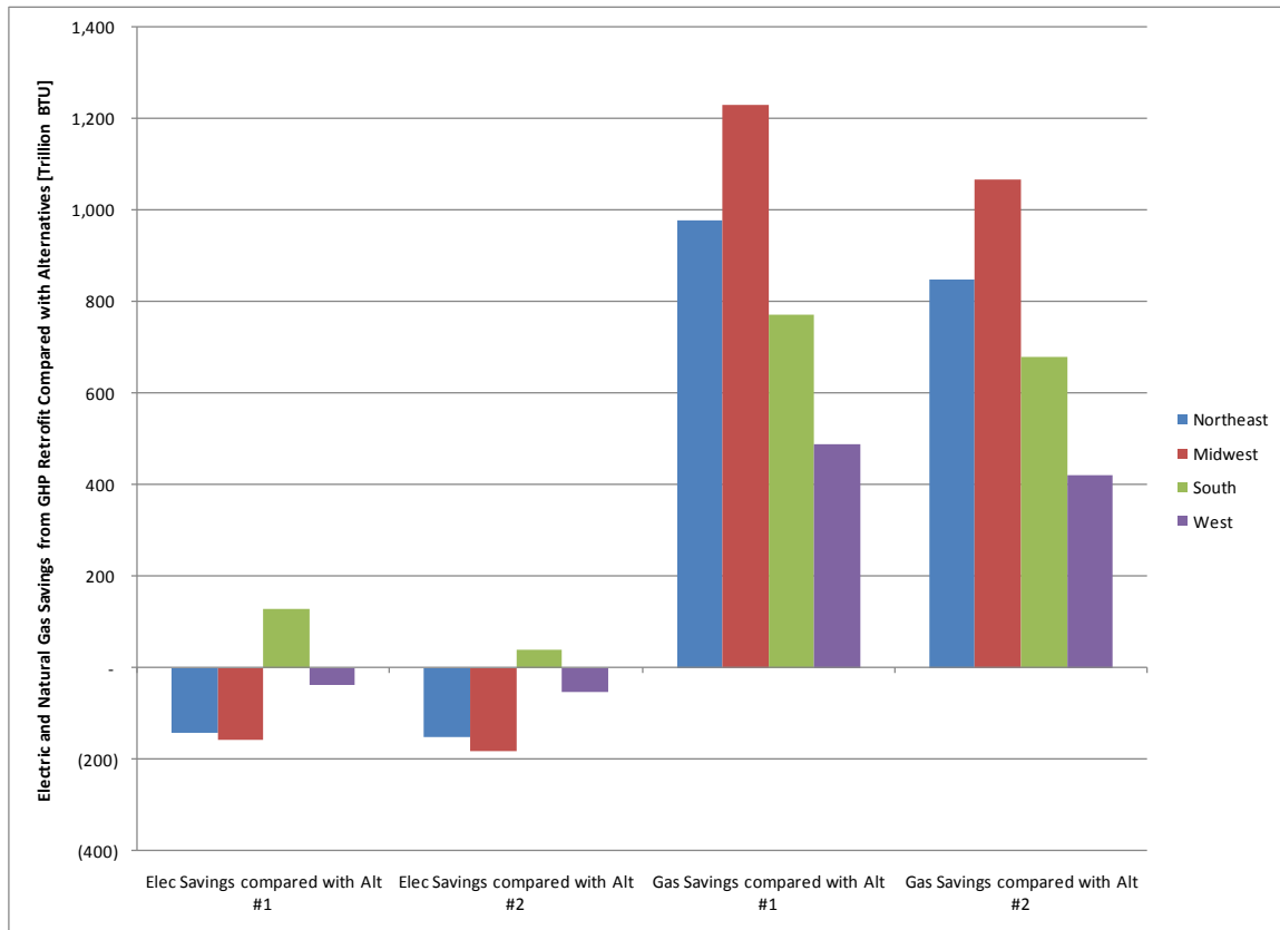
Fig. 5. Saved electricity and natural gas from GHP retrofits vs. alternatives in each census region.
