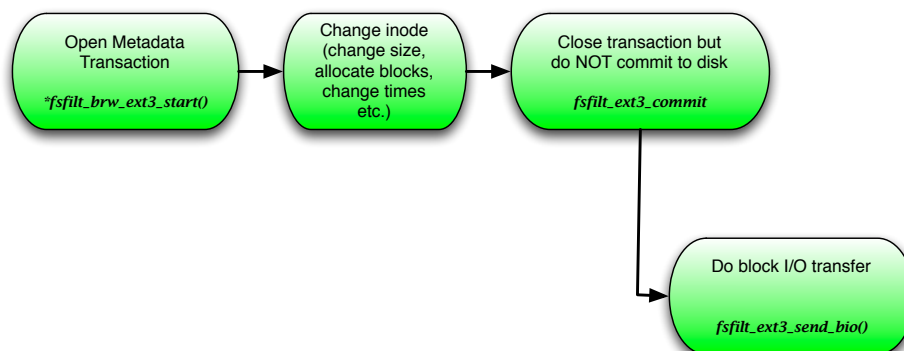
Figure 17: Fsfilt flow path for asynchronous block I/O operations.
