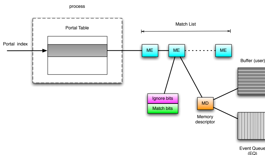
Figure 12: Illustration of Lustre LNET addressing scheme.
