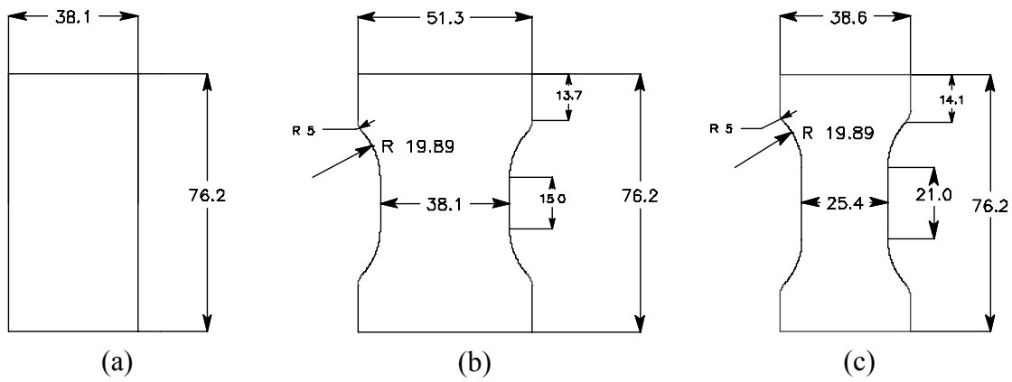
Figure 2. Sample Geometries for Initial Compression Testing (dimensions in mm)
