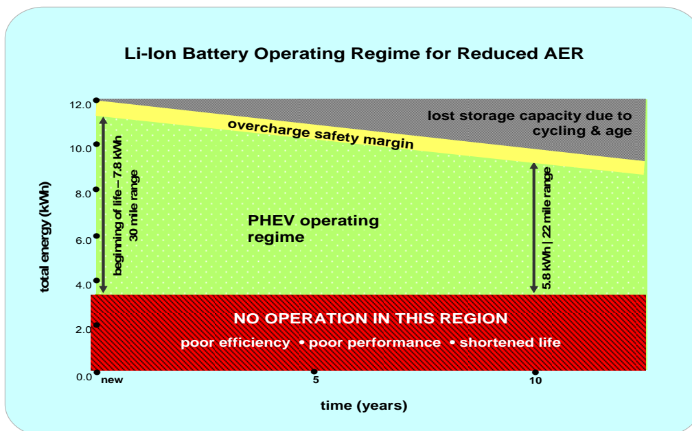
Figure 19: Potential battery pack conceptual design without reserve capacity to accommodate cycling and aging losses.
